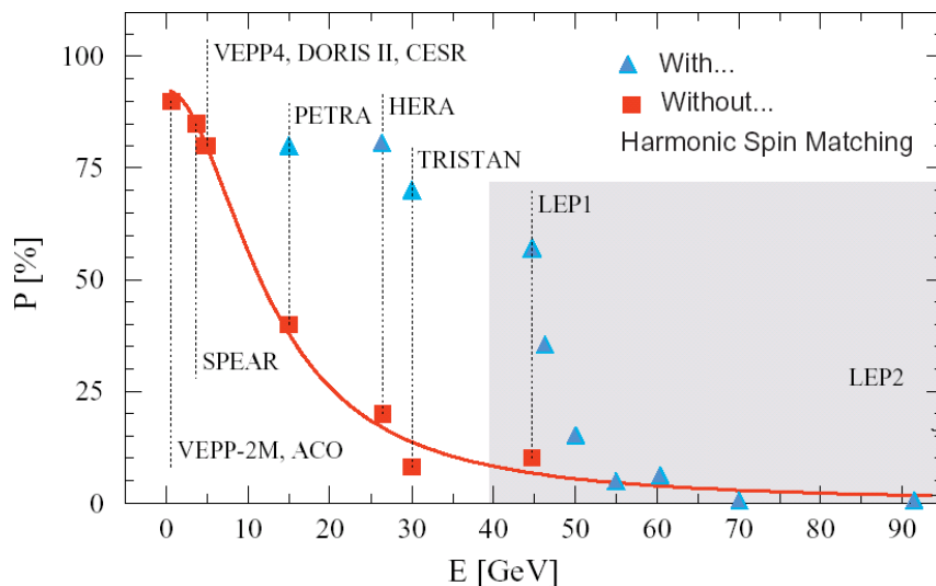
Figure 4.2: Electron polarization levels achieved in various circular circular electron storage rings [15].
