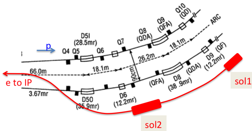
Figure 4.3: Layout of the electron spin rotators.
