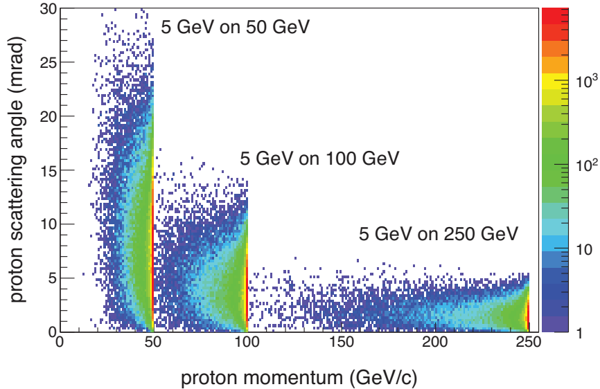
Figure 3.1: The scattered proton momentum versus scattering angle in the laboratory frames for deeply virtual Compton scattering (DVCS) events with different beam energy combinations. The following cuts have been applied: 1 \text{ GeV}^2 < Q^2 < 100 \text{ GeV}^2 , 0.00001 < x < 0.7 and 0 < t < 2 \text{ GeV}^2 . The angle of the recoiling hadronic system is directly and inversely correlated with the proton energy. It thus decreases with increasing proton energy.
