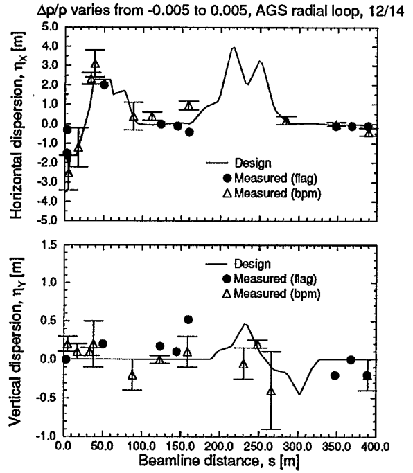
Figure 2: Dispersion functions of the ATR as measured by varying the AGS extraction energy.
