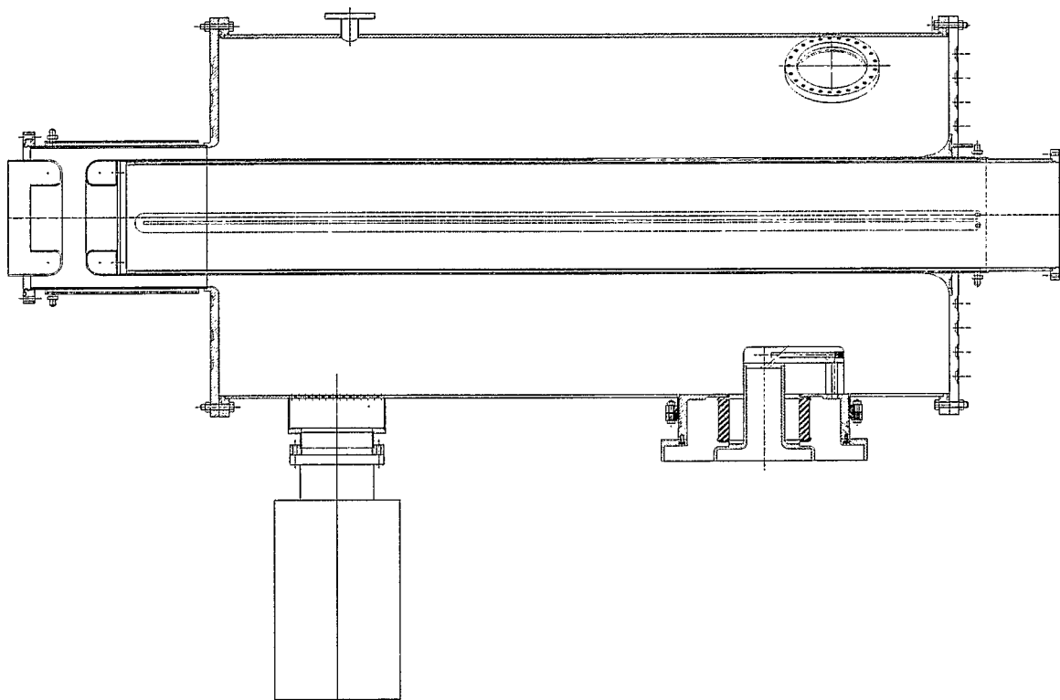
Figure 7.7: Accelerating cavity
