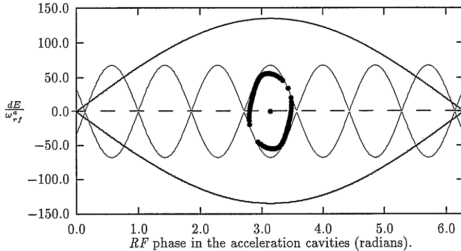
Figure 5.3: Dashed line is the bucket in 26MHz bucket, solid line is the storage bucket, dots are representative particles. \epsilon = 0.3 eVs/u , V_{rf,a}^a = 300 kV , V_{rf,s}^s = 550 kV
