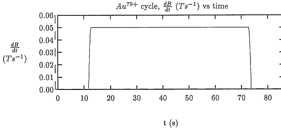
Figure 7.1: \frac{dB}{dt} program.
