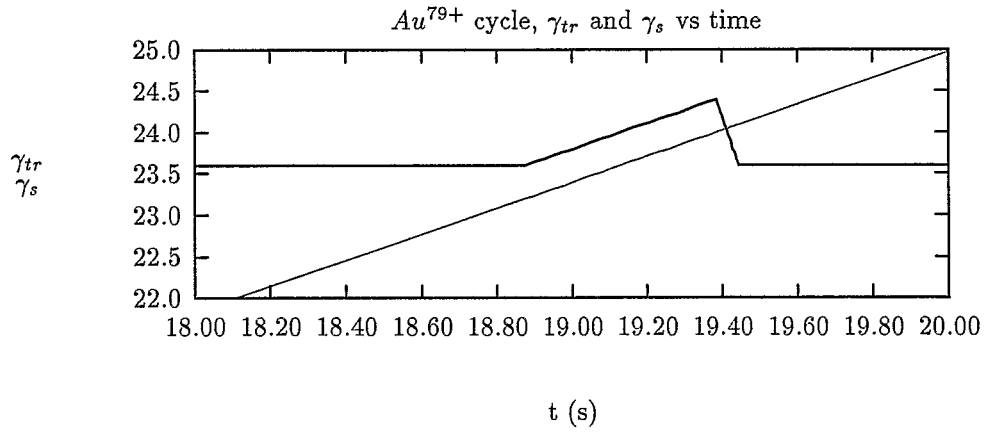
Figure 7.4: \gamma_{tr} jump region.
