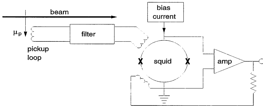
FIGURE 3. Block Diagram
