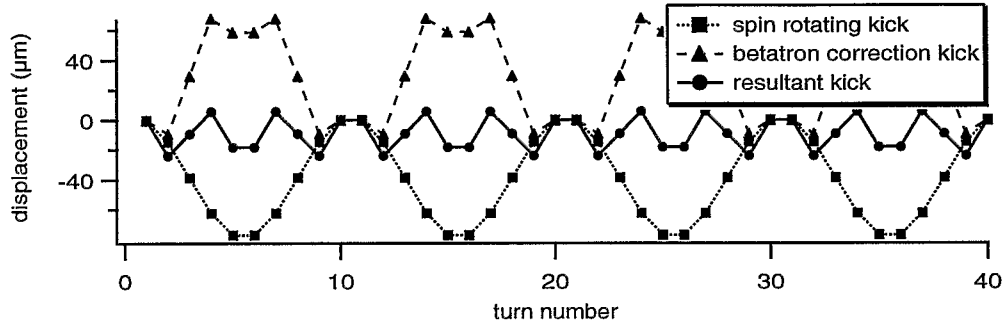
FIGURE 1. Beam Displacement due to Spin Flipping and Correction
