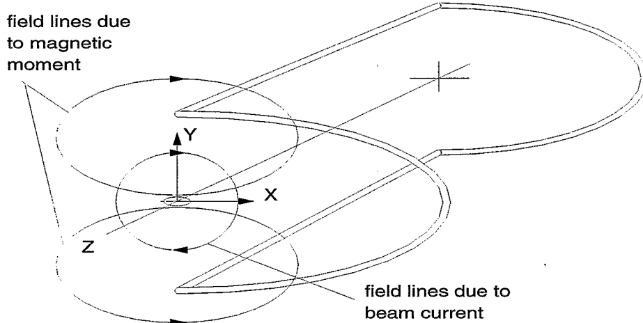
FIGURE 2. The Pickup Loop
