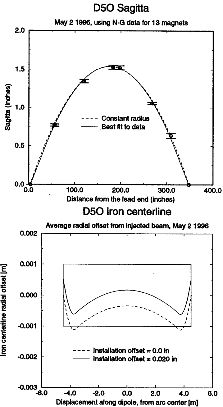
Figure 5: Sagitta data and fit, and centerline offset, for D5O dipoles.
