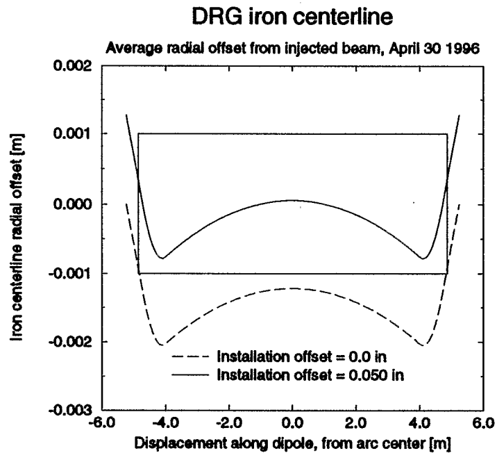
Figure 2: Sagitta data and fit, and centerline offset, for DRG dipoles.
