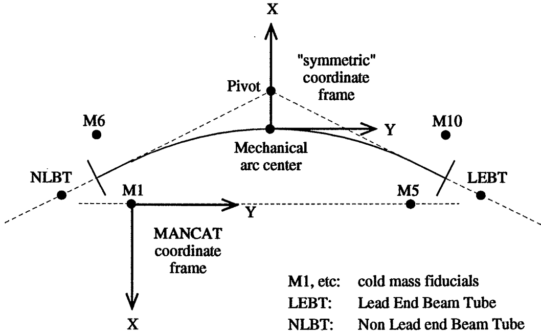
Figure 7: Origins and orientations of the two local coordinate frames, the “symmetric” frame and the “MANCAT” frame.
