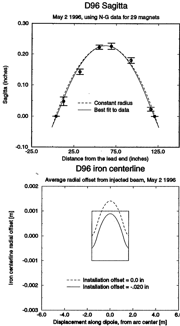
Figure 6: Sagitta data and fit, and centerline offset, for D96 dipoles.
