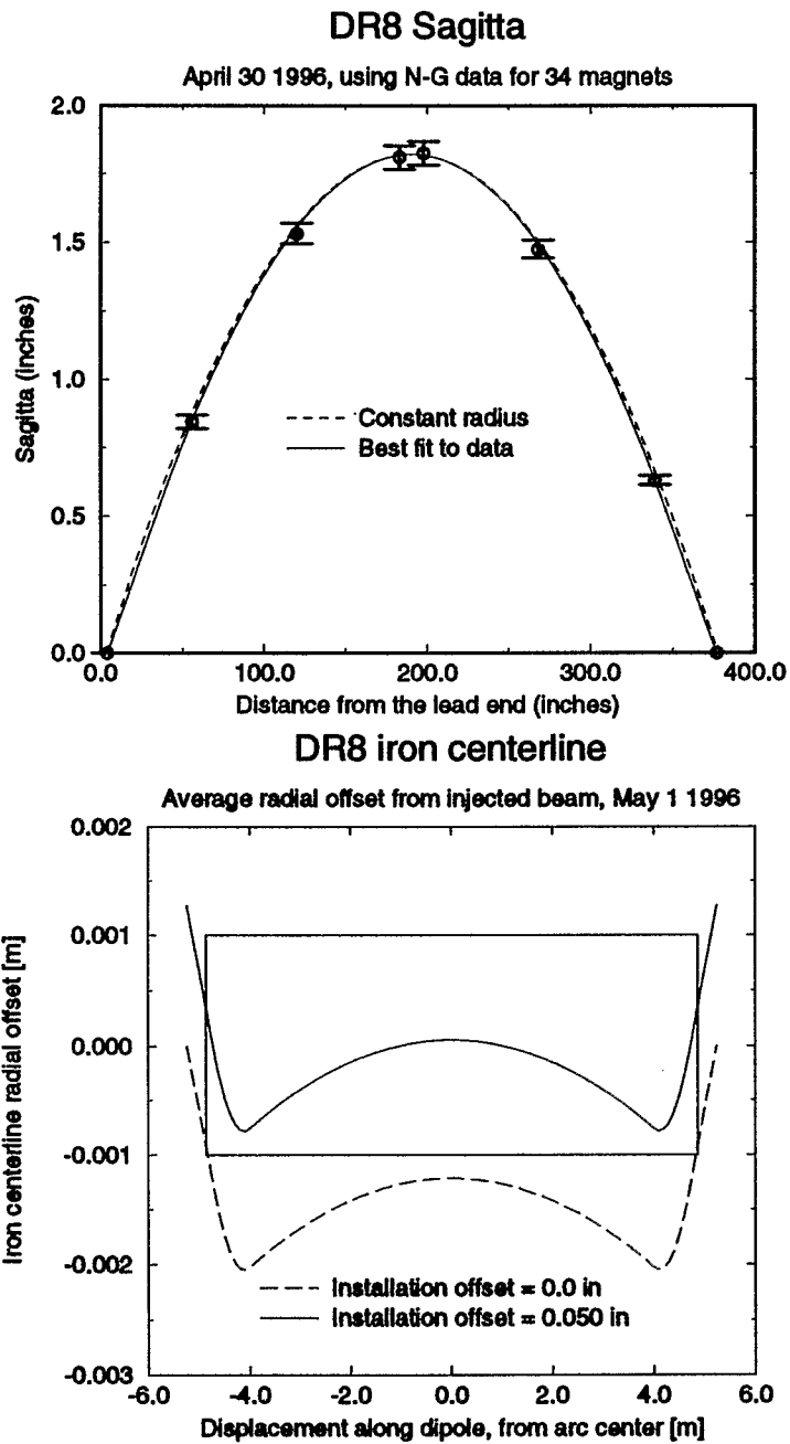
Figure 3: Sagitta data and fit, and centerline offset, for DR8 dipoles.
