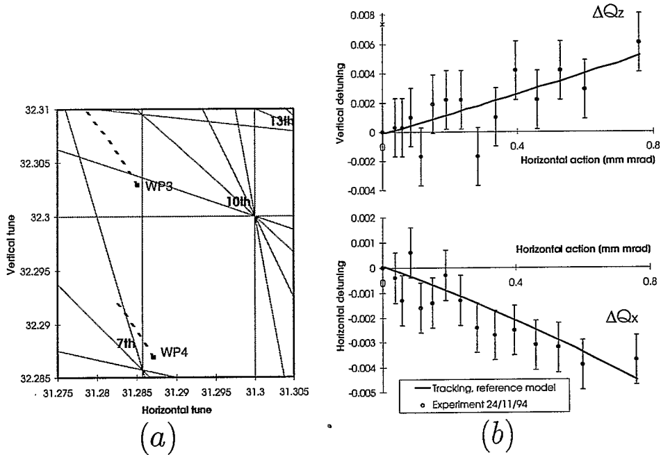
FIGURE 4: (a) The working points WP3 and WP4 in the tune diagram. Sum resonances up to order 13 are shown. The dotted lines show the detuning when the horizontal dynamic aperture is approached. (b) Detuning of the HERA proton ring at working point WP3 with the set-up given in Tab 1.
