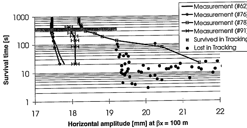
FIGURE 3: Dynamic aperture at WP1, tune modulation of 9Hz and \Delta Q_x = 1.87 \cdot 10^{-3} .
