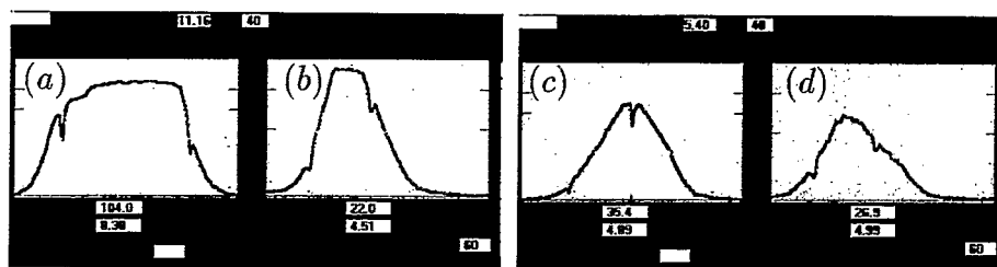
FIGURE 5: Beam profiles at two different times after a horizontal kick with a beam of 60 bunches. Part (a) and (b) show the horizontal and vertical beam profile respectively right after the kick, the horizontal profile (c) and the vertical profile (d) were taken 10 minutes later. The notches are markers to determine the width of the profile.
