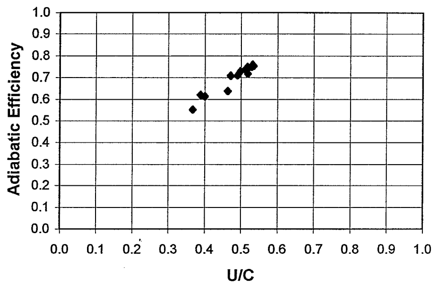
Figure 2 Efficiency of Turbine 1B2 as a function of U/C
