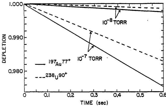
Fig. II-3. Depletion of beam in the AGS.
