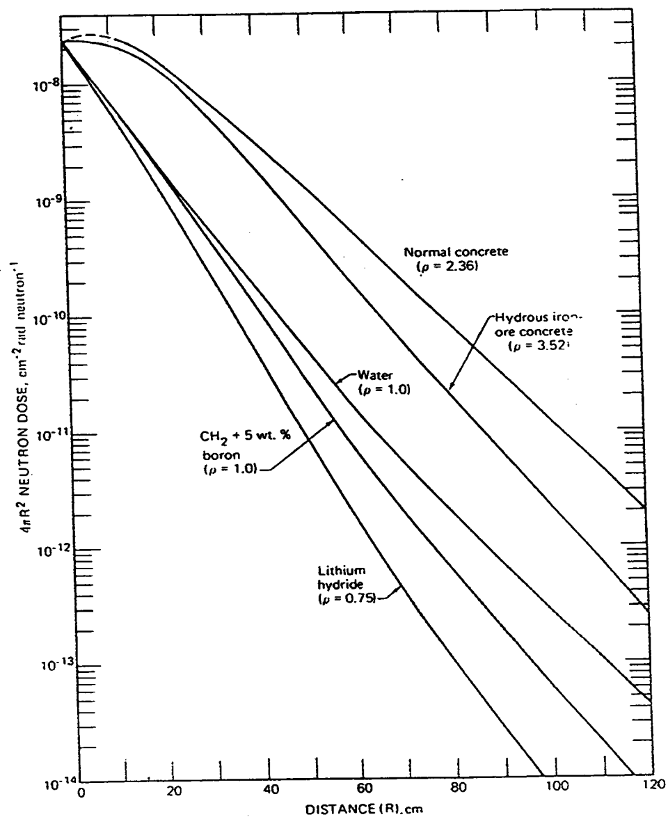
Fig. 8.12—Neutron dose vs. depth in the indicated materials fission-neutron source. (Based on data from Nichols 47 and Kam and Clark. 48 )
