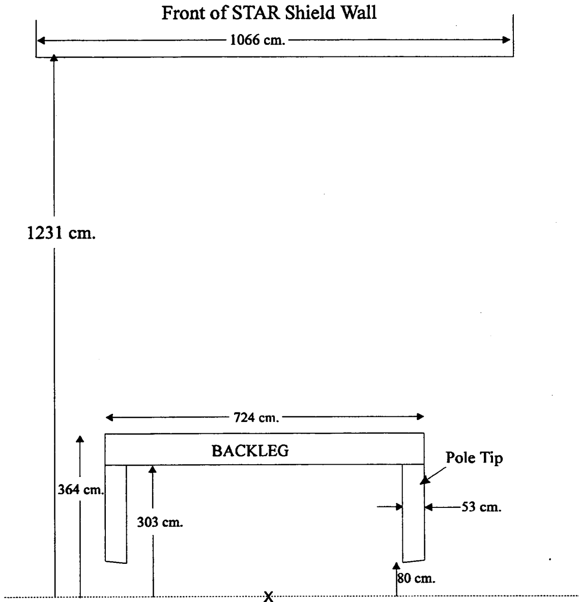
Fig. 1 Approximation of The STAR Detector
