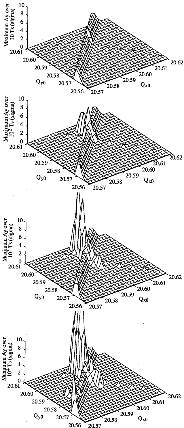
Figure 5: Maximum vertical amplitudes of single particles with initial amplitudes (a_x, a_y) = (3.0, 0.1)\sigma , tracked for 10, 10^2 , 10^3 and 10^4 synchrotron periods.
