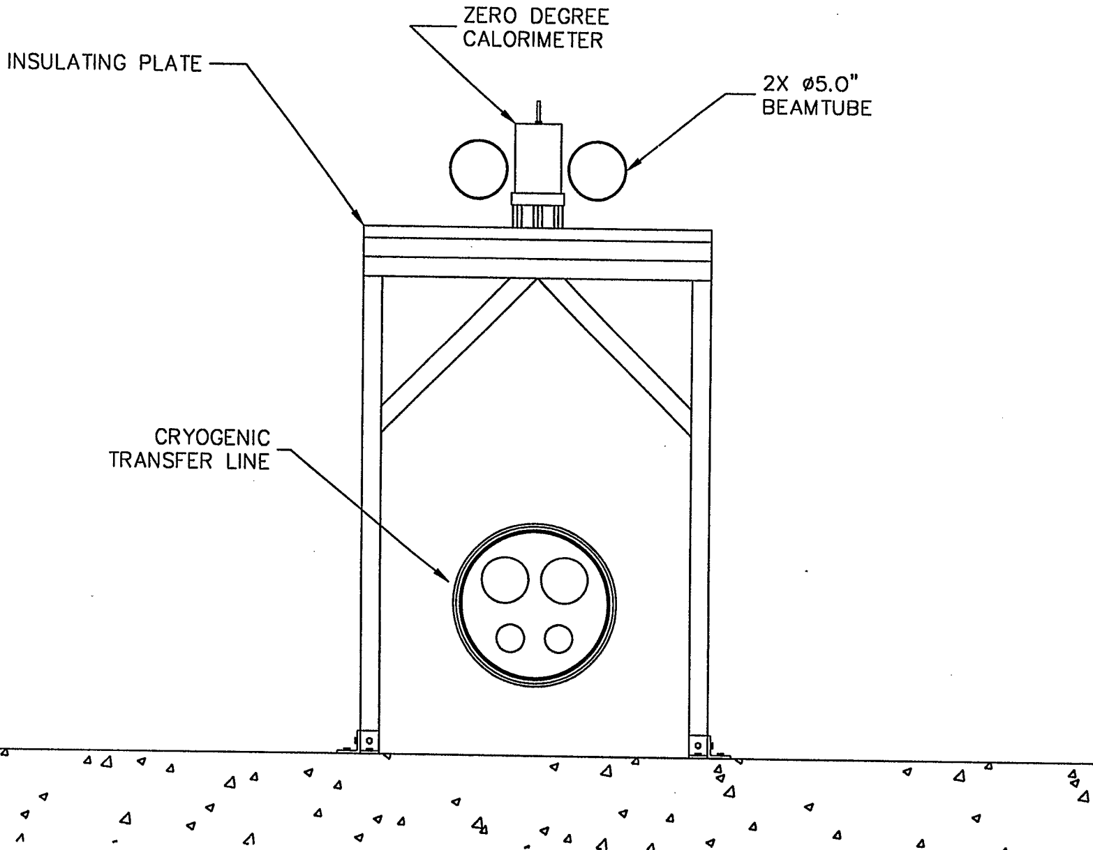
FRONT VIEW
