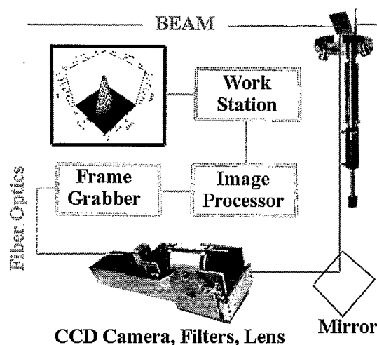
Figure 1: Beam Profile Monitor System
