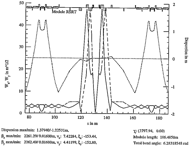
Figure 4: the IR with two FMC modules of the 50 GeV isochronous demon muon collider lattice.
