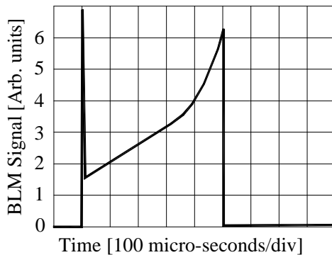
Figure 5b. The schematic version shows an injection momentum loss not present in the actual PSR losses, but, aside from being inverted, it looks very much like the actual loss.
