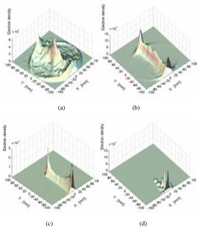
Figure 6: Electron distribution with 2000Volts clearing potentials at different time. (a) 350 ns, (b) 560 ns, (c) 630 ns and (d) 700 ns.
