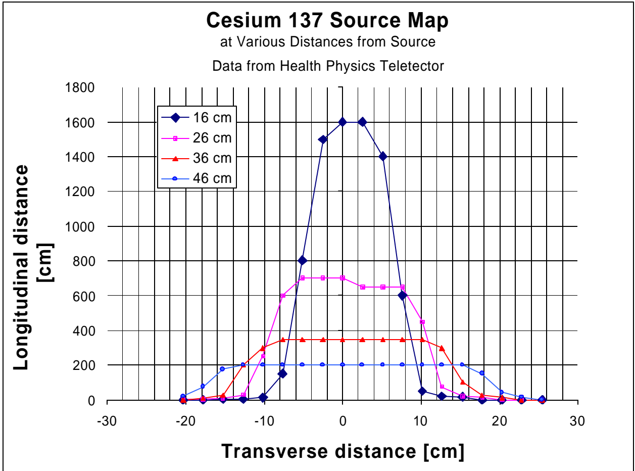
Figure 1. Plot of Cesium 137 source transverse distribution.
