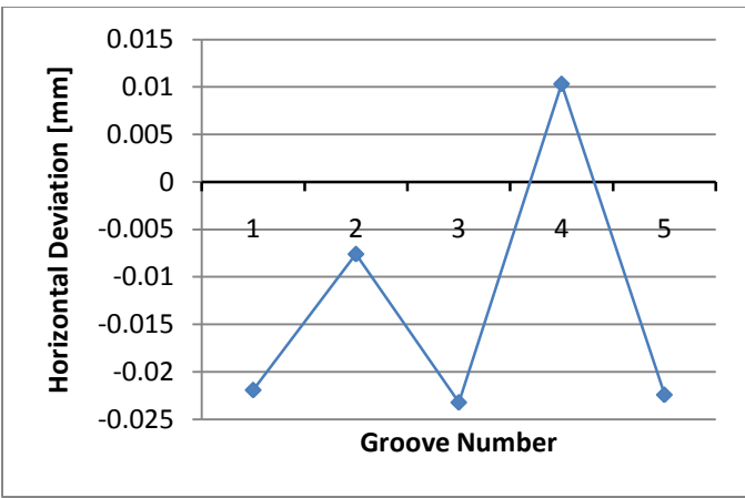
Figure 43: 360-degree orientation for inner grooves using camera.
