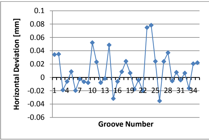
Figure 45: Deviations for cavity choke joint using camera.
