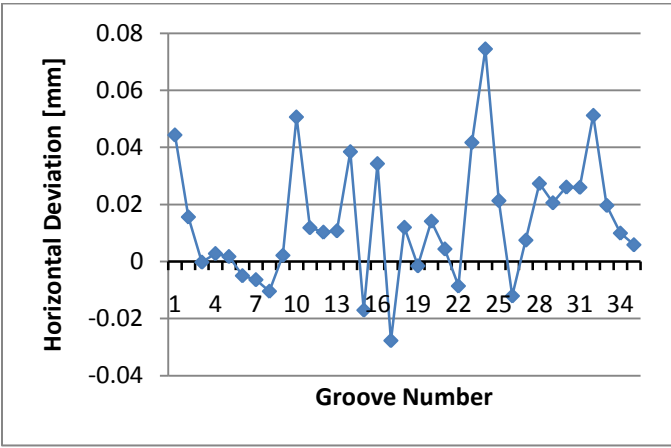
Figure 44: Deviations for cavity choke joint using articulated arm.
