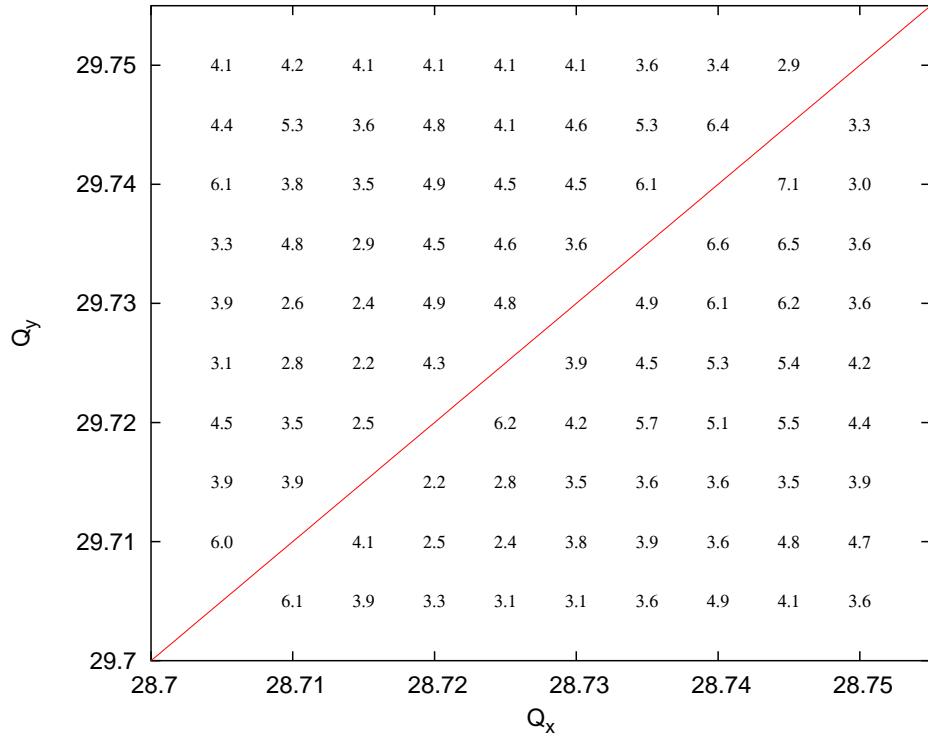
Figure 14: DAs in the tune scan above 0.7 under condition of (IRcorr + BB + b2 +2fam ).
