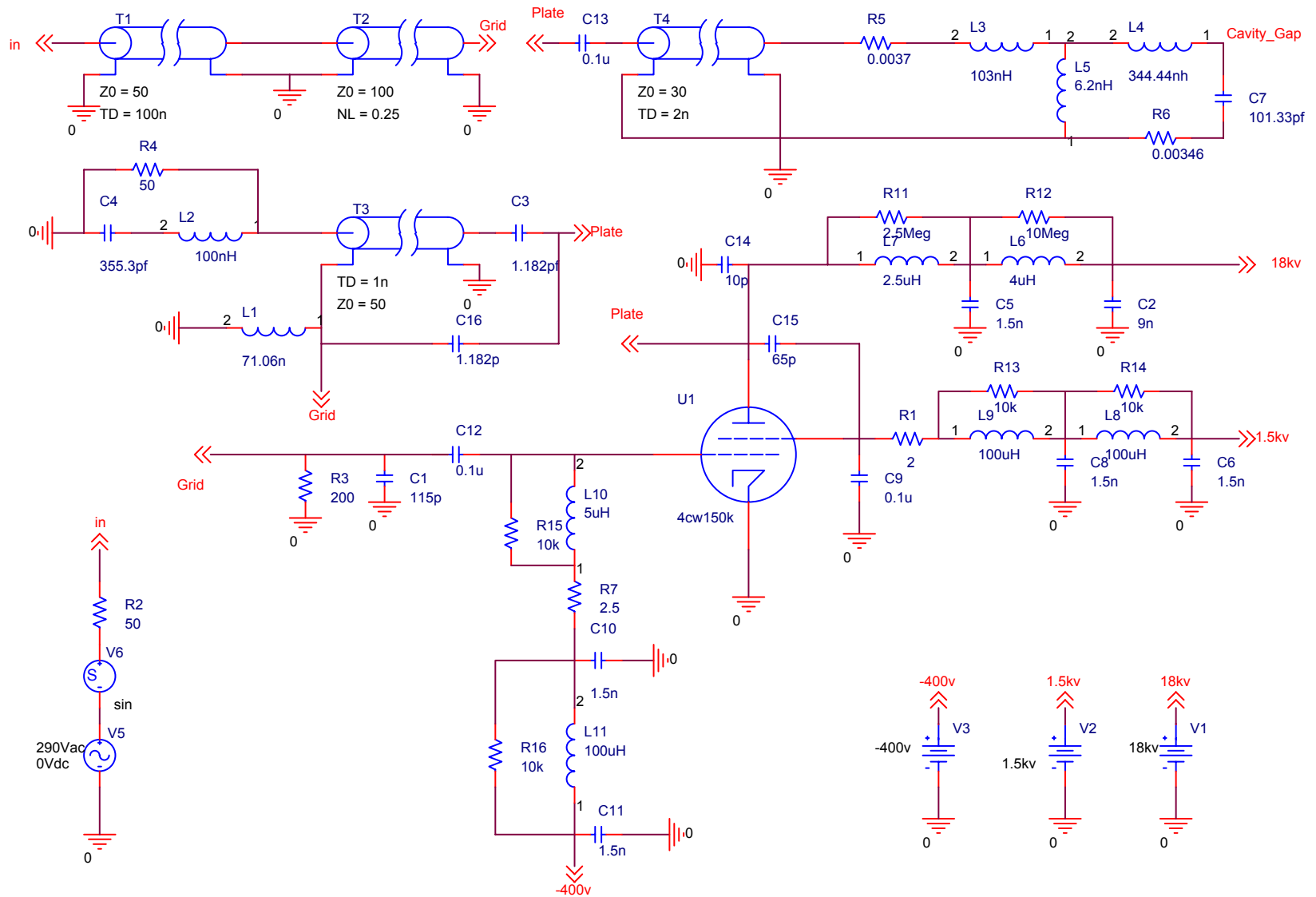
Fig. 7 A PSPICE model of the 28 MHz PA for the accelerating cavity.
