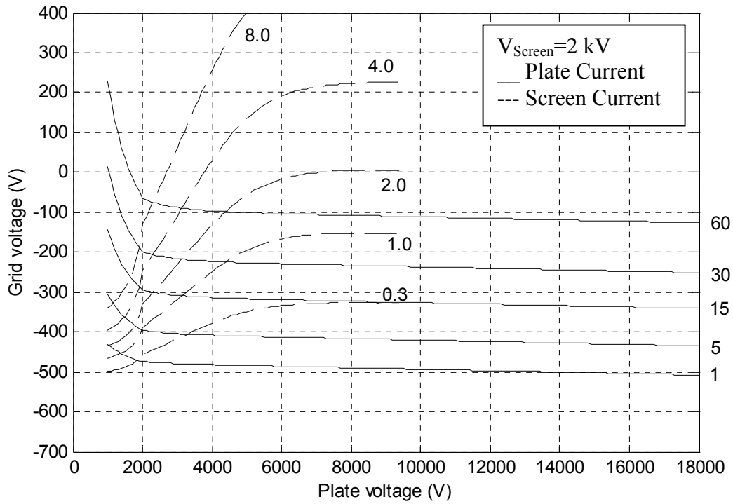
Fig. 4. Constant-current curves ( V_{\text{Screen}} = 2 \text{ kV} ) from the Tetrode model
