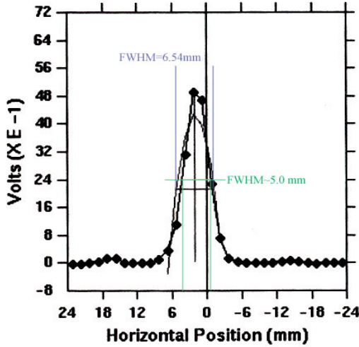
Figure 3: MW006 horizontal profile with parabolic fit for narrow beam. Note that FWHM from parabolic fit (6.54mm) is larger than that obtained visually from the graph (~5.0 mm). Wires are 1.5 mm apart.
