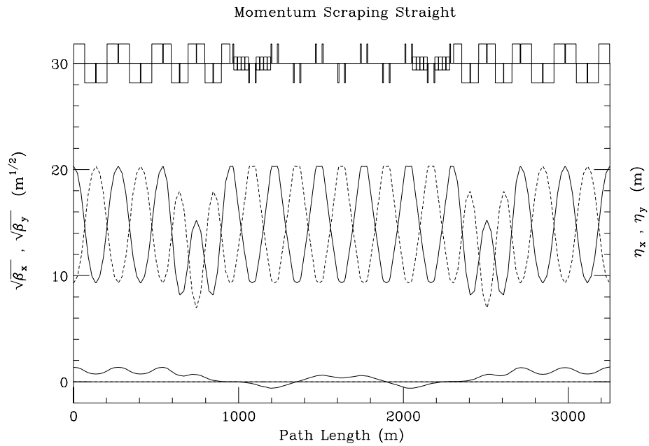
Figure 13: Dispersion creation in a 5-cell straight for collimation.
