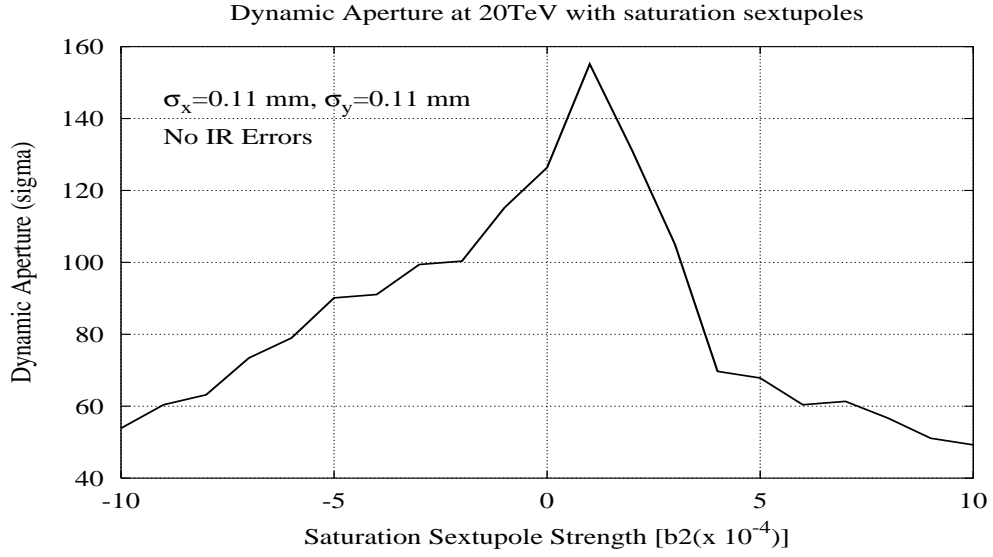
Figure 19: Dynamic aperture at top energy as a function of the saturation b_2 in the arc magnets without field errors in the IR quadrupoles.
