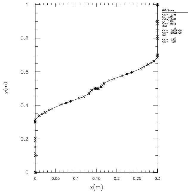
Figure 66: Trajectory of the 10 TeV transfer line from Stage 1 to Stage 2 rings.
