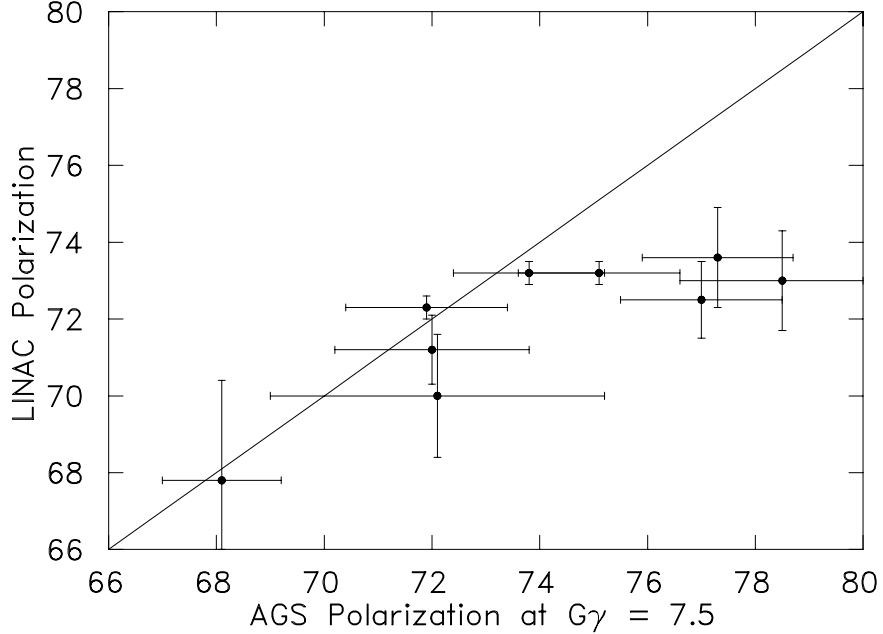
FIG. 3: Comparison of polarization measured at 200 MeV and at G\gamma = 7.5 . The horizontal error bars indicate only the statistical error in the corresponding asymmetry measurement, because that is the only independent error between the data points. The exception is the point farthest to the left, which corresponds to the initial measurement to which all other points are calibrated. In this case the error bar indicates the systematic error which is common to the other points but which is actually not an error in the measurement of the calibration point; in other words it indicates the amount by which the other points could vary in unison with respect to the calibration point. The vertical error bars indicate statistical errors only.
