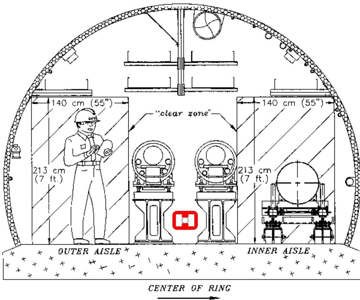
Figure 2: RHIC tunnel cross-section, showing an electron ring magnet between the ion ring stands.
