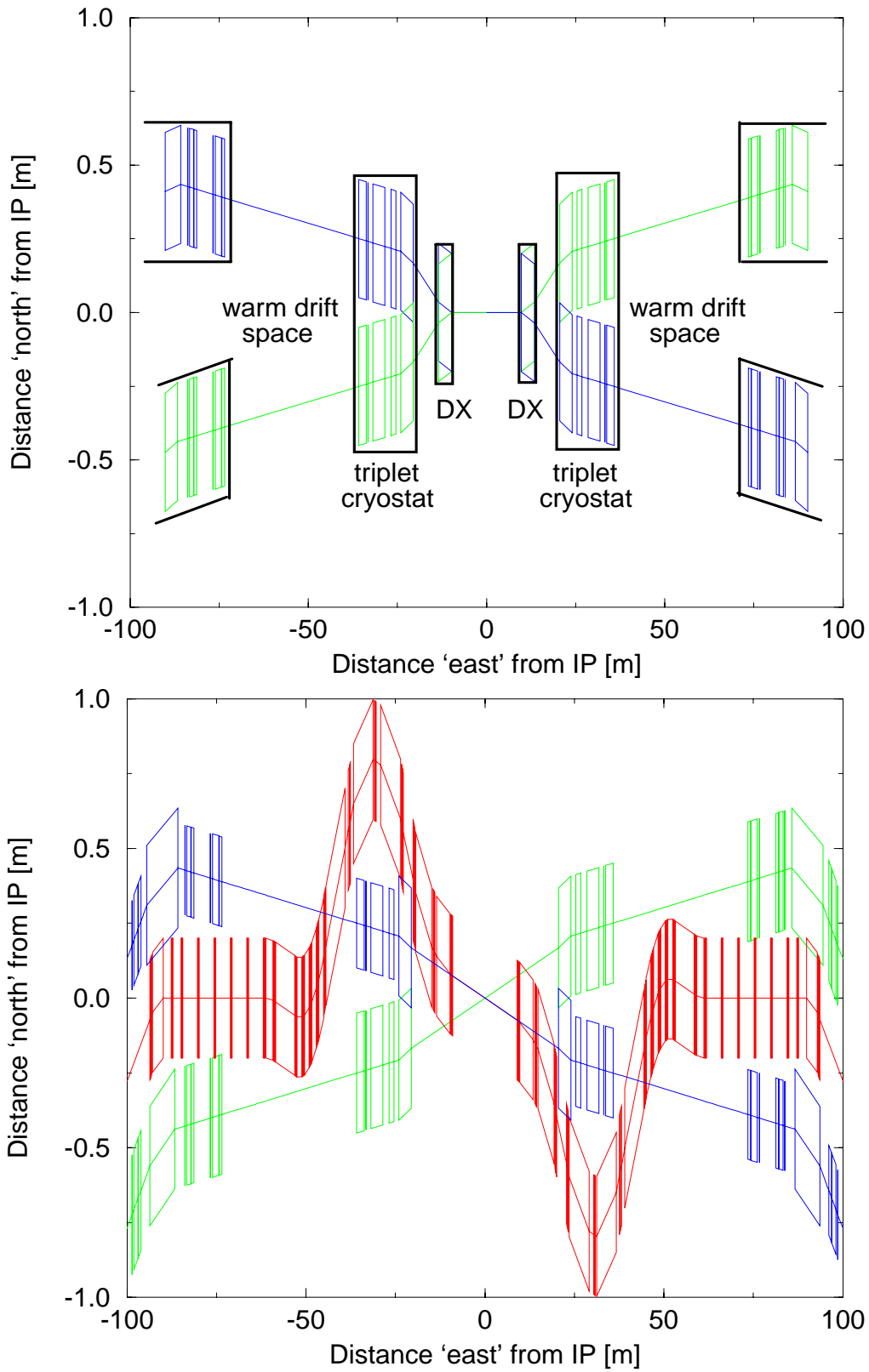
Figure 6: The magnet layout close to the IP in nominal RHIC operation during gold-gold or proton-proton collisions (top), and after modification for eRHIC (bottom).
