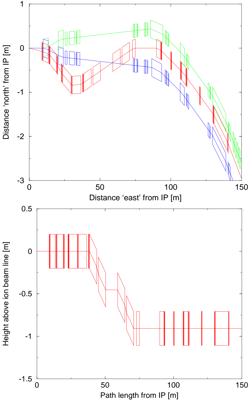
Figure 7: Plan and side views of the eRHIC magnet layout in an interaction region WITHOUT spin rotators.
