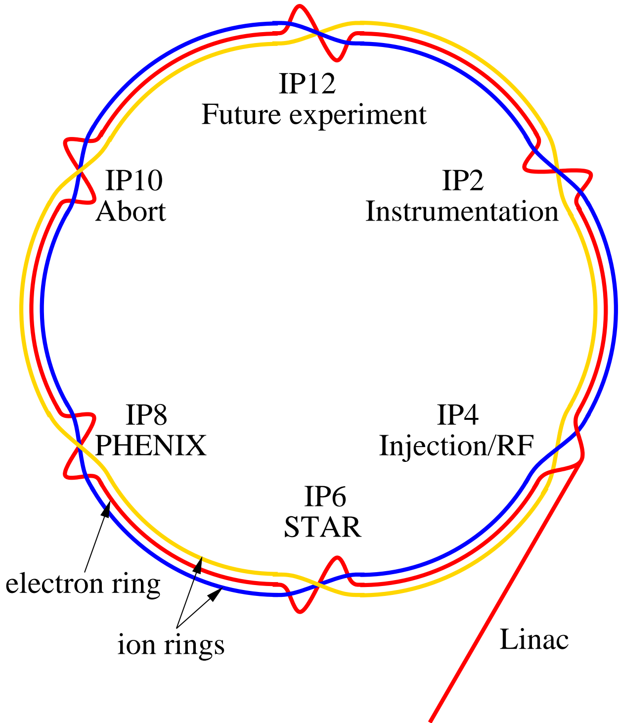
Figure 1: Schematic layout of the injection linac, electron ring, and the two ion rings, in the ring-ring collision scenario.
