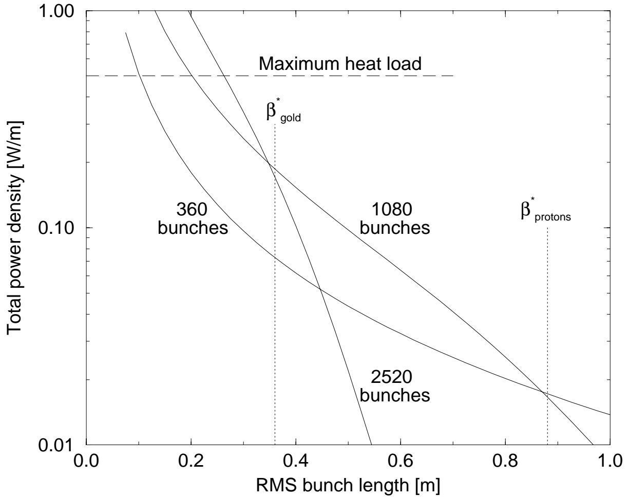
Figure 11: Linear power load deposited at cryogenic temperatures in the stainless steel vacuum chamber of the ion rings, due to beam image currents, for a total charge of 0.93 \times 10^{11} per bunch – at the beam-beam limit for the electrons.
