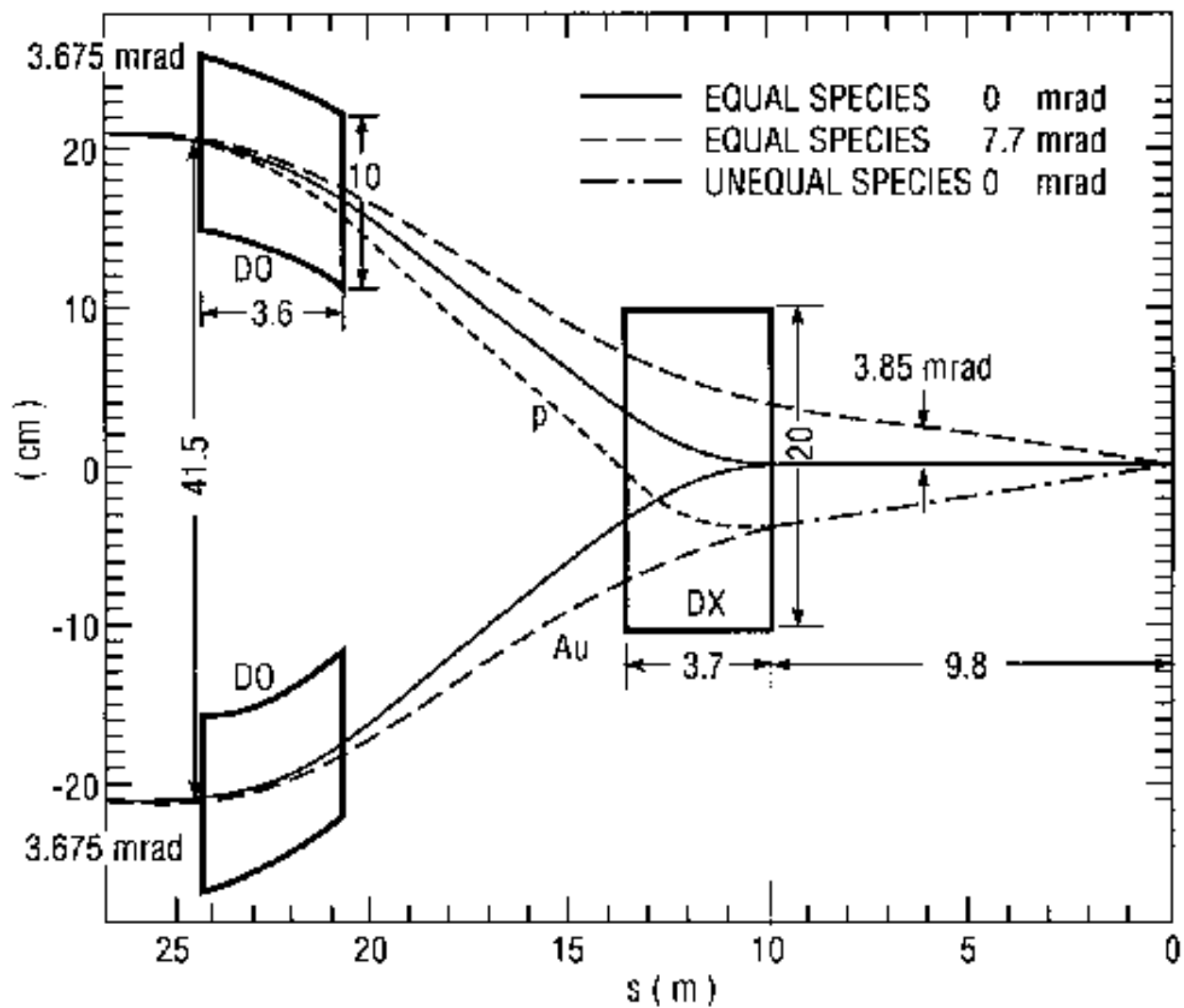
Figure 5: Nominal layout at the interaction region, showing a common crossing angle of 3.85 mrad during proton-gold collisions.
