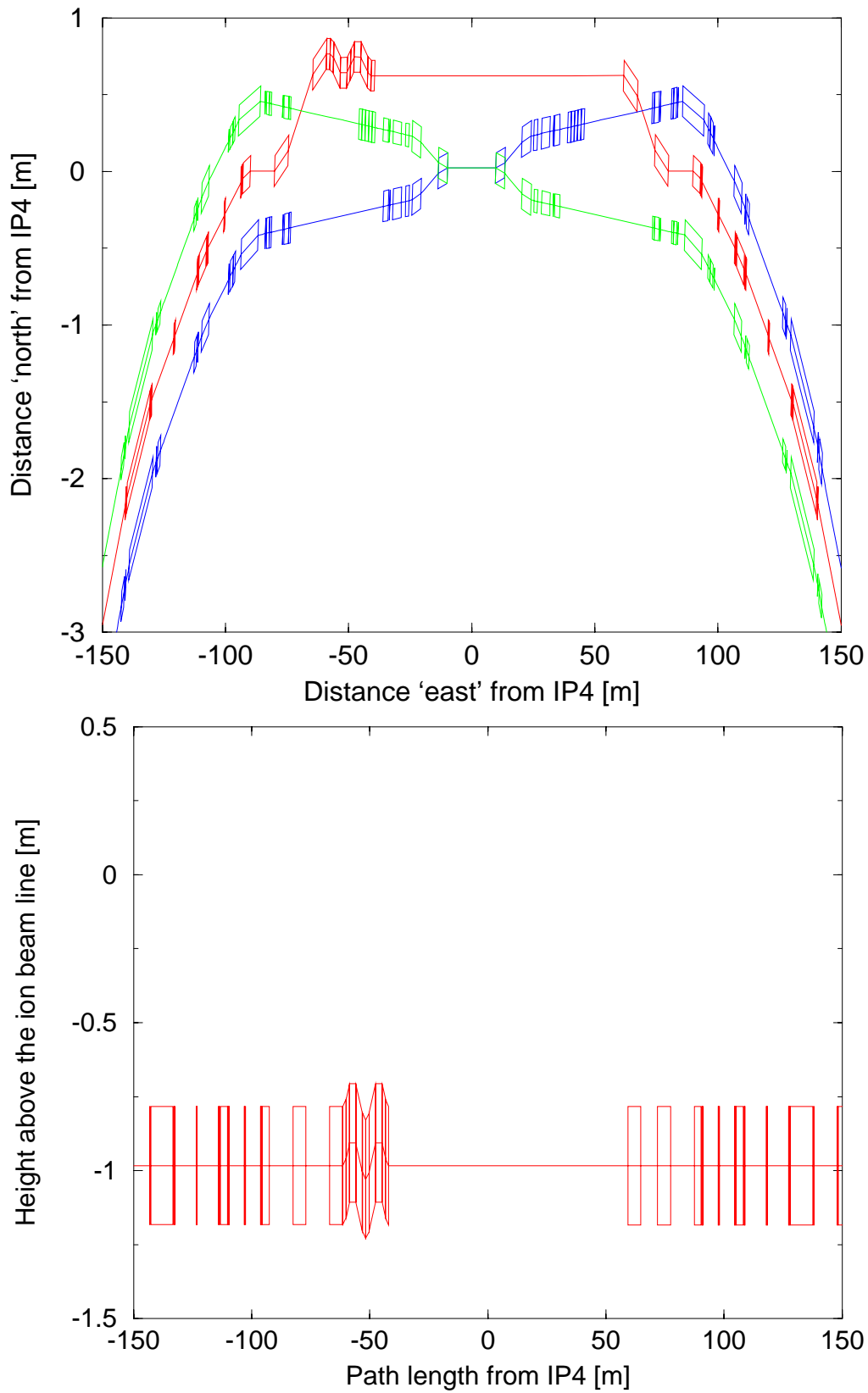
Figure 10: Plan and side views of the magnetic layout around the utility region IP4, including a Siberian snake of the first kind.
