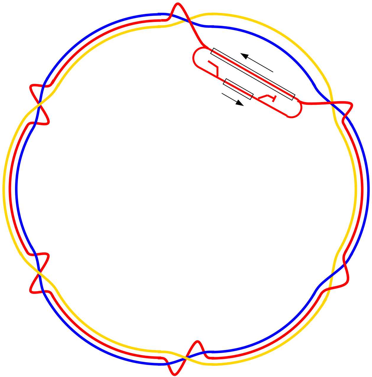
Figure 4: Schematic layout for linac-ring collisions, using the RHIC tunnel to return the 10 GeV electrons for energy recovery.
