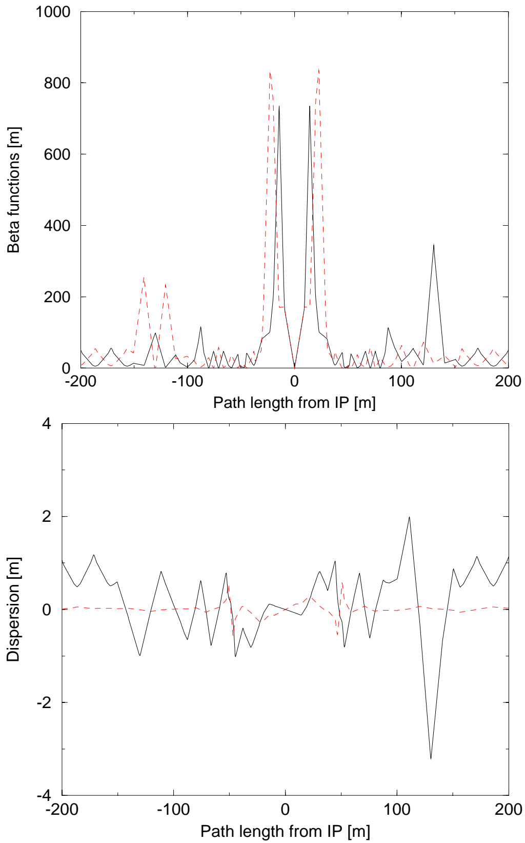
Figure 9: Beta and dispersion functions around an IP with spin rotators.
