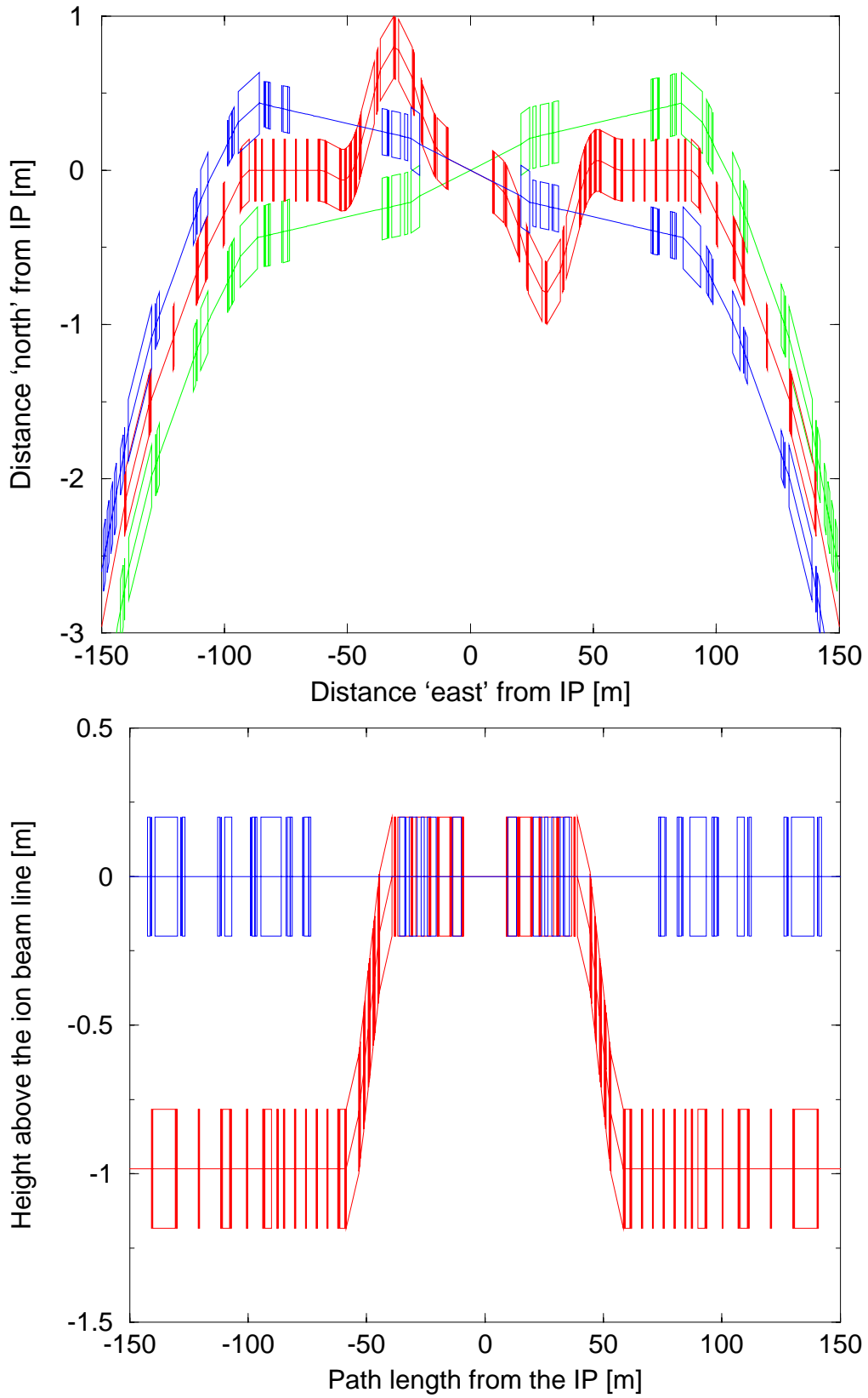
Figure 8: Plan and side views of the eRHIC magnet layout in an interaction region WITH spin rotators.
