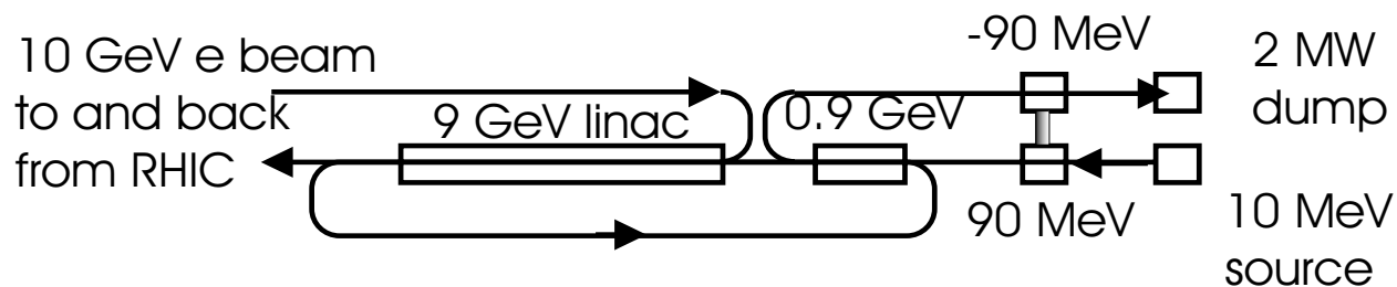
Figure 3: Schematic layout of a two stage recirculating linac structure in the linac-ring collision scenario.
