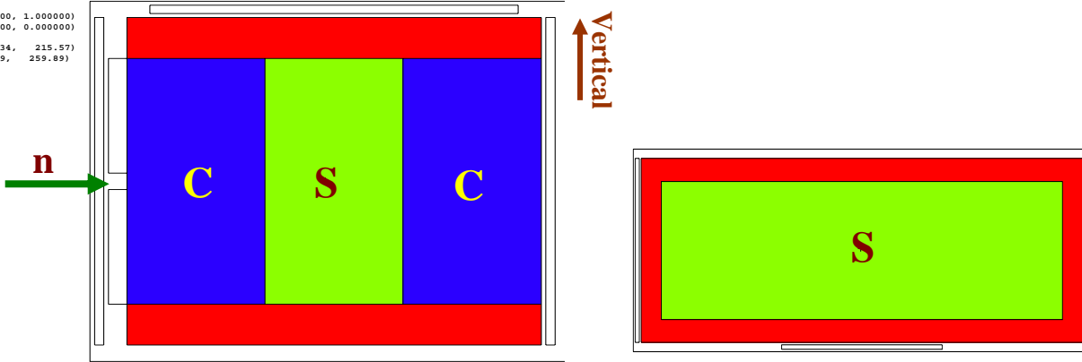
Figure 1: Left : The beam dump with configuration CSC (concrete-steel-concrete) along the beam direction. The four sides are covered by light concrete. The colorless/empty blocks (as seen in the figure) are empty volumes defined in the MCNPX which are the places where radiation levels are calculated. The arrow gives the direction of the incoming neutrons. Right : The cross-sectional (in the XY plane perpendicular to the beam direction) view of the beam dump. The four sides are covered by light concrete.
