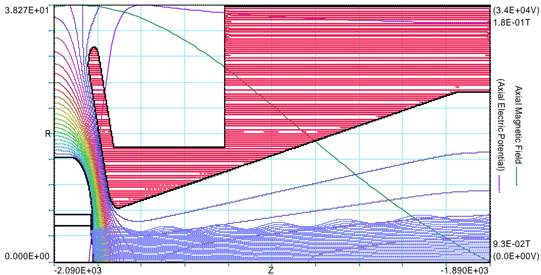
Fig. 11. Simulated electron trajectories for a high perveance version of the gun electrodes with shielded Wehnelt electrode. I_{el} = 20 A, U_{an} = 38273 V, P = 2.67 \times 10^{-6} \text{ A/V}^{3/2} .
