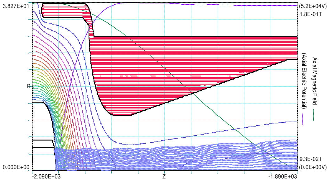
Fig. 7. Simulated electron trajectories with a prototype geometry of the gun electrodes. I_{el} = 20 A, U_{an} = 56329 V, P = 1.49 \times 10^{-6} A/V 3/2 .
