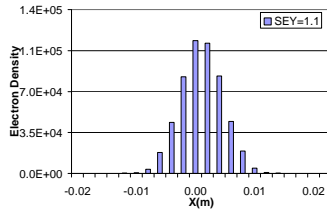
Figure 1. Electron cloud distribution in RHIC dipole field for B = 0.334 T and SEY = 1.1, bunch length=1.2 m.
