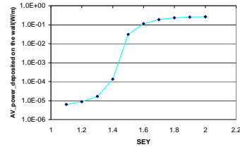
Figure 45. Electron cloud average power deposited on the wall vs SEY at transition in the RHIC dipole chamber.
