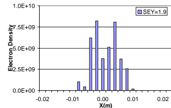
Figure 43. Electron cloud distribution in RHIC dipole field for B = 0.845 T and SEY = 1.9, bunch length=0.5 m.
