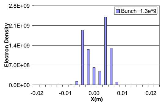
Figure 55. EC distribution in RHIC dipole field for B = 0.845 T and SEY = 1.5, bunch intensity = 1.3 \times 10^9 .
