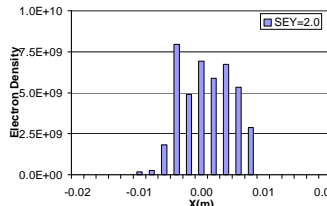
Figure 21. Electron cloud distribution in RHIC dipole field for B = 0.334 T and SEY = 2.0, bunch length = 0.6 m.
