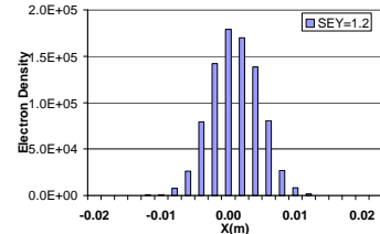
Figure 36. Electron cloud distribution in RHIC dipole field for B = 0.845 T and SEY = 1.2, bunch length=0.5 m.
