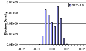
Figure 42. Electron cloud distribution in RHIC dipole field for B = 0.845 T and SEY = 1.8, bunch length = 0.5 m.
