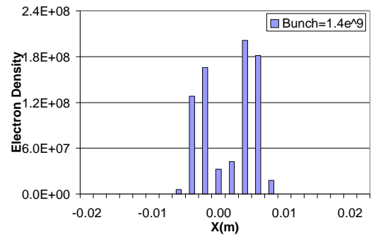
Figure 50. EC distribution in RHIC dipole field for B = 0.845 T and SEY = 1.4, bunch intensity = 1.4 \times 10^9 .
