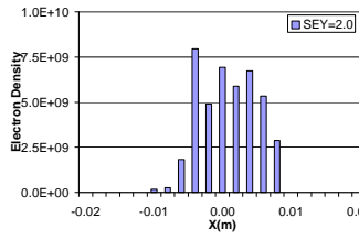
Figure 21. Electron cloud distribution in RHIC dipole field for B = 0.334 T and SEY = 2.0, bunch length=0.6 m.
