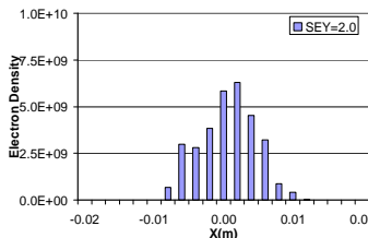
Figure 5. Electron cloud distribution in RHIC dipole field for B = 0.334 T and SEY = 2.0, bunch length=1.2 m.
