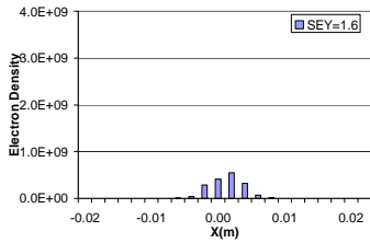
Figure 1. Electron cloud distribution in RHIC dipole field for B = 0.334 T and SEY = 1.6, bunch length=1.2 m.
