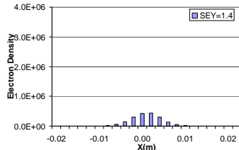
Figure 4. Electron cloud distribution in RHIC dipole field for B = 0.334 T and SEY = 1.4, bunch length=1.2 m.
