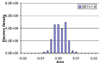
Figure 3. Electron cloud distribution in RHIC dipole field for B = 0.334 T and SEY = 1.8, bunch length=1.2 m.
