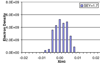
Figure 18. Electron cloud distribution in RHIC dipole field for B = 0.334 T and SEY = 1.7, bunch length = 0.6 m.
