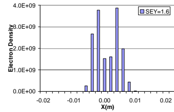
Figure 40. Electron cloud distribution in RHIC dipole field for B = 0.845 T and SEY = 1.6, bunch length=0.5 m.
