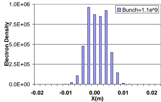
Figure 47. EC distribution in RHIC dipole field for B = 0.845 T and SEY = 1.4, bunch intensity = 1.1 \times 10^9 .
