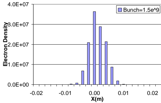
Figure 34. EC distribution in RHIC dipole field for B = 0.334 T and SEY = 1.5, bunch intensity = 1.5 \times 10^9 .
