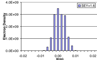
Figure 17. Electron cloud distribution in RHIC dipole field for B = 0.334 T and SEY = 1.6, bunch length = 0.6 m.
