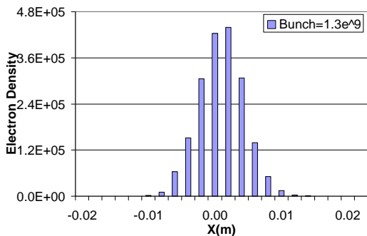
Figure 26. EC distribution in RHIC dipole field for B = 0.334 T and SEY = 1.4, bunch intensity = 1.3 \times 10^9 .
