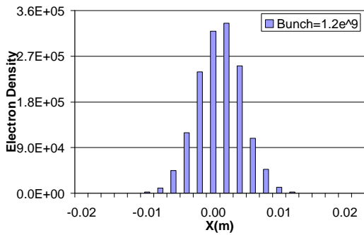
Figure 25. EC distribution in RHIC dipole field for B = 0.334 T and SEY = 1.4, bunch intensity = 1.2 \times 10^9 .
