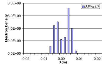
Figure 41. Electron cloud distribution in RHIC dipole field for B = 0.845 T and SEY = 1.7, bunch length=0.5 m.
