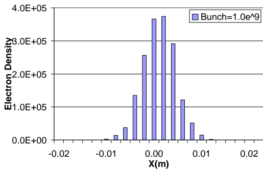
Figure 29. EC distribution in RHIC dipole field for B = 0.334 T and SEY = 1.5, bunch intensity = 1.0 \times 10^9 .
