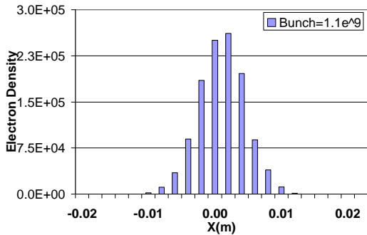
Figure 24. EC distribution in RHIC dipole field for B = 0.334 T and SEY = 1.4, bunch intensity = 1.1 \times 10^9 .
