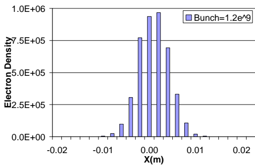
Figure 31. EC distribution in RHIC dipole field for B = 0.334 T and SEY = 1.5, bunch intensity = 1.2 \times 10^9 .
