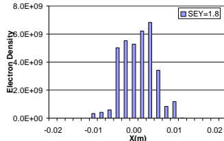
Figure 19. Electron cloud distribution in RHIC dipole field for B = 0.334 T and SEY = 1.8, bunch length = 0.6 m.
