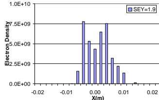
Figure 20. Electron cloud distribution in RHIC dipole field for B = 0.334 T and SEY = 1.9, bunch length = 0.6 m.
