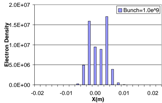
Figure 52. EC distribution in RHIC dipole field for B = 0.845 T and SEY = 1.5, bunch intensity = 1.0 \times 10^9 .
