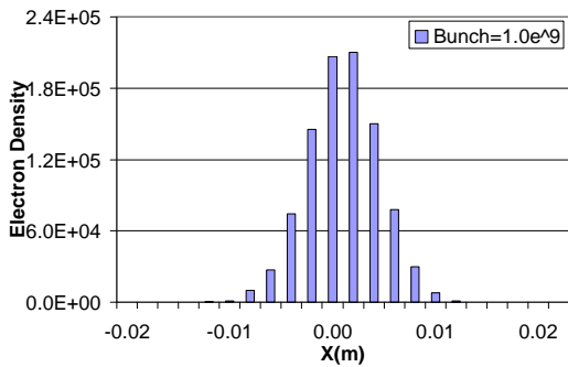
Figure 23. EC distribution in RHIC dipole field for B = 0.334 T and SEY = 1.4, bunch intensity = 1.0 \times 10^9 .
