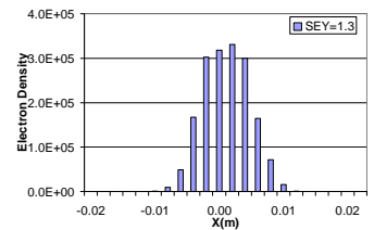
Figure 37. Electron cloud distribution in RHIC dipole field for B = 0.845 T and SEY = 1.3, bunch length=0.5 m.
