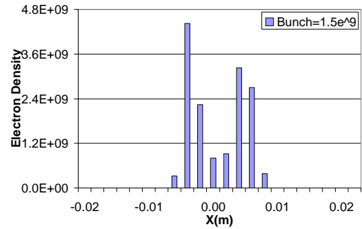
Figure 57. EC distribution in RHIC dipole field for B = 0.845 T and SEY = 1.5, bunch intensity = 1.5 \times 10^9 .
