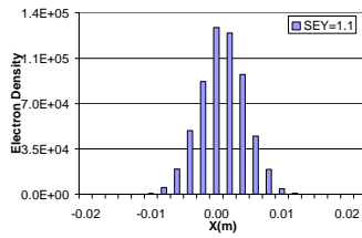
Figure 12. Electron cloud distribution in RHIC dipole field for B = 0.334 T and SEY = 1.1, bunch length=0.6 m.
