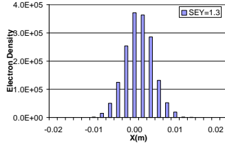
Figure 14. Electron cloud distribution in RHIC dipole field for B = 0.334 T and SEY = 1.3, bunch length=0.6 m.
