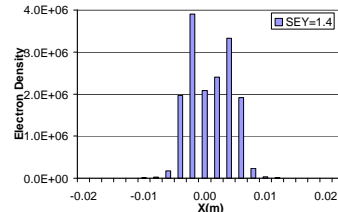
Figure 38. Electron cloud distribution in RHIC dipole field for B = 0.845 T and SEY = 1.4, bunch length=0.5 m.
