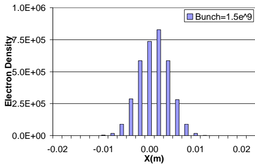
Figure 28. EC distribution in RHIC dipole field for B = 0.334 T and SEY = 1.4, bunch intensity = 1.5 \times 10^9 .
