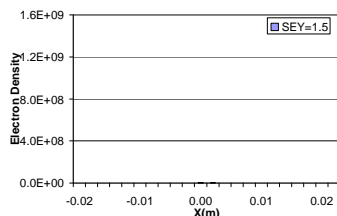
Figure 5. Electron cloud distribution in RHIC dipole field for B = 0.334 T and SEY = 1.5, bunch length=1.2 m.
