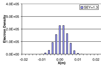
Figure 3. Electron cloud distribution in RHIC dipole field for B = 0.334 T and SEY = 1.3, bunch length=1.2 m.
