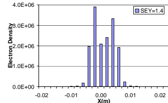
Figure 38. Electron cloud distribution in RHIC dipole field for B = 0.845 T and SEY = 1.4, bunch length=0.5 m.
