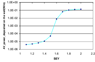
Figure 11. Electron cloud average power deposited on the chamber wall vs SEY at injection, bunch length = 1.2 m.
