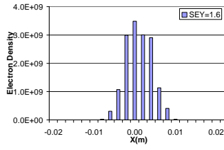
Figure 17. Electron cloud distribution in RHIC dipole field for B = 0.334 T and SEY = 1.6, bunch length=0.6 m.
