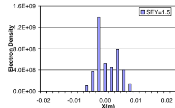
Figure 39. Electron cloud distribution in RHIC dipole field for B = 0.845 T and SEY = 1.5, bunch length=0.5 m.
