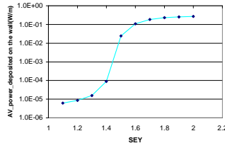
Figure 22. Electron cloud average power deposited on the chamber wall vs SEY at injection, bunch length = 0.6 m.
