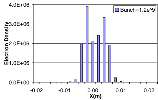
Figure 48. EC distribution in RHIC dipole field for B = 0.845 T and SEY = 1.4, bunch intensity = 1.2 \times 10^9 .
