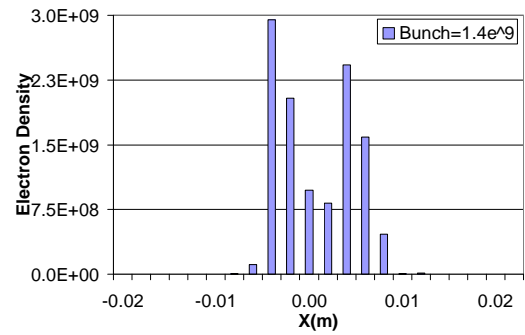
Figure 56. EC distribution in RHIC dipole field for B = 0.845 T and SEY = 1.5, bunch intensity = 1.4 \times 10^9 .
