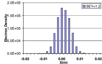
Figure 36. Electron cloud distribution in RHIC dipole field for B = 0.845 T and SEY = 1.2, bunch length=0.5 m.
