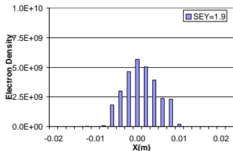
Figure 4. Electron cloud distribution in RHIC dipole field for B = 0.334 T and SEY = 1.9, bunch length=1.2 m.
