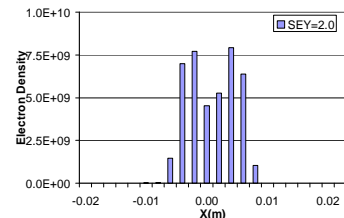
Figure 44. Electron cloud distribution in RHIC dipole field for B = 0.845 T and SEY = 2.0, bunch length=0.5 m.
