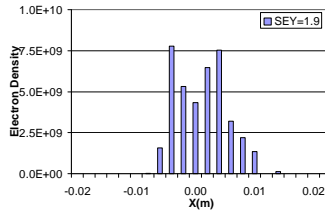
Figure 20. Electron cloud distribution in RHIC dipole field for B = 0.334 T and SEY = 1.9, bunch length=0.6 m.
