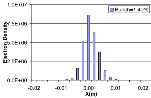
Figure 33. EC distribution in RHIC dipole field for B = 0.334 T and SEY = 1.5, bunch intensity = 1.4 \times 10^9 .
