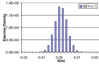
Figure 12. Electron cloud distribution in RHIC dipole field for B = 0.334 T and SEY = 1.1, bunch length=0.6 m.
