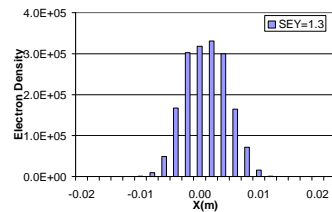
Figure 37. Electron cloud distribution in RHIC dipole field for B = 0.845 T and SEY = 1.3, bunch length=0.5 m.
