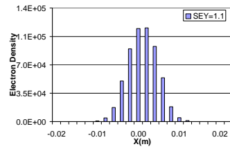
Figure 35. Electron cloud distribution in RHIC dipole field for B = 0.845 T and SEY = 1.1, bunch length=0.5 m.
