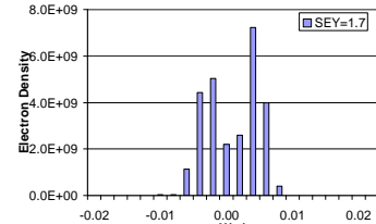
Figure 41. Electron cloud distribution in RHIC dipole field for B = 0.845 T and SEY = 1.7, bunch length = 0.5 m.
