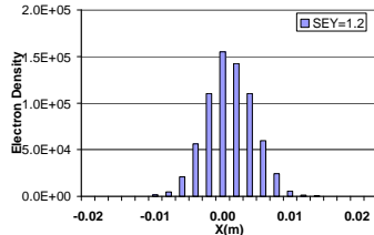
Figure 2. Electron cloud distribution in RHIC dipole field for B = 0.334 T and SEY = 1.2, bunch length=1.2 m.
