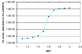
Figure 11. Electron cloud average power deposited on the chamber wall vs SEY at injection, bunch length = 1.2 m.
