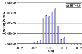
Figure 19. Electron cloud distribution in RHIC dipole field for B = 0.334 T and SEY = 1.8, bunch length=0.6 m.
