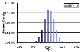
Figure 1. Electron cloud distribution in RHIC dipole field for B = 0.334 T and SEY = 1.1, bunch length=1.2 m.
