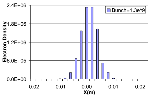
Figure 32. EC distribution in RHIC dipole field for B = 0.334 T and SEY = 1.5, bunch intensity = 1.3 \times 10^9 .
