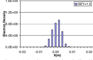
Figure 16. Electron cloud distribution in RHIC dipole field for B = 0.334 T and SEY = 1.5, bunch length=0.6 m.
