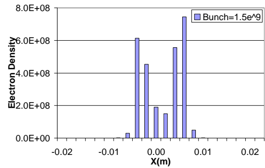
Figure 51. EC distribution in RHIC dipole field for B = 0.845 T and SEY = 1.4, bunch intensity = 1.5 \times 10^9 .
