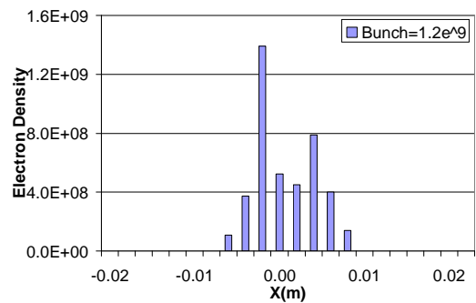
Figure 54. EC distribution in RHIC dipole field for B = 0.845 T and SEY = 1.5, bunch intensity = 1.2 \times 10^9 .
