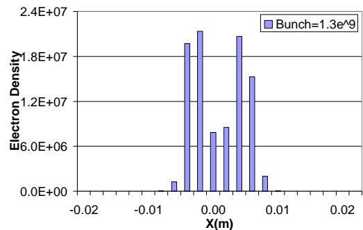
Figure 49. EC distribution in RHIC dipole field for B = 0.845 T and SEY = 1.4, bunch intensity = 1.3 \times 10^9 .
