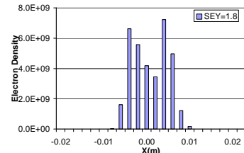
Figure 42. Electron cloud distribution in RHIC dipole field for B = 0.845 T and SEY = 1.8, bunch length=0.5 m.
