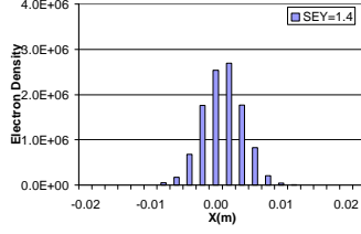
Figure 15. Electron cloud distribution in RHIC dipole field for B = 0.334 T and SEY = 1.4, bunch length=0.6 m.
