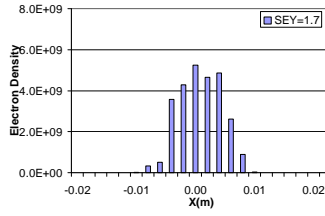
Figure 18. Electron cloud distribution in RHIC dipole field for B = 0.334 T and SEY = 1.7, bunch length=0.6 m.
