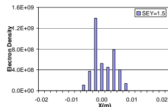
Figure 39. Electron cloud distribution in RHIC dipole field for B = 0.845 T and SEY = 1.5, bunch length=0.5 m.
