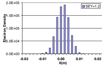
Figure 13. Electron cloud distribution in RHIC dipole field for B = 0.334 T and SEY = 1.2, bunch length=0.6 m.
