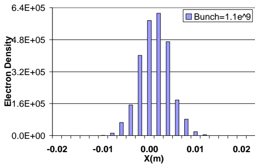
Figure 30. EC distribution in RHIC dipole field for B = 0.334 T and SEY = 1.5, bunch intensity = 1.1 \times 10^9 .
