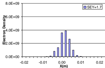
Figure 2. Electron cloud distribution in RHIC dipole field for B = 0.334 T and SEY = 1.7, bunch length=1.2 m.
