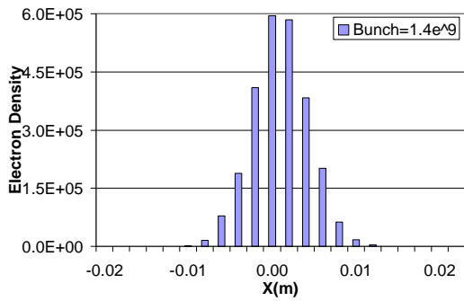
Figure 27. EC distribution in RHIC dipole field for B = 0.334 T and SEY = 1.4, bunch intensity = 1.4 \times 10^9 .
