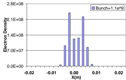
Figure 53. EC distribution in RHIC dipole field for B = 0.845 T and SEY = 1.5, bunch intensity = 1.1 \times 10^9 .
