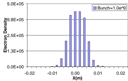
Figure 46. EC distribution in RHIC dipole field for B = 0.845 T and SEY = 1.4, bunch intensity = 1.0 \times 10^9 .
