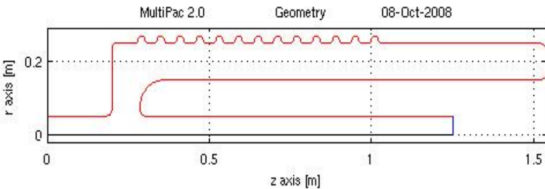
Fig. 9. Ripple pointing towards upward direction.
