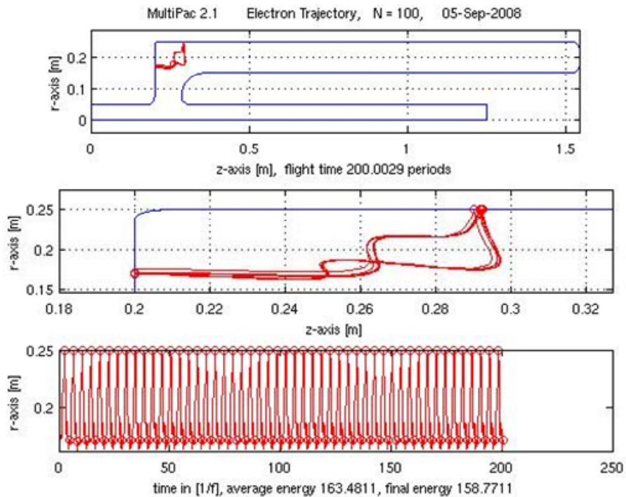
Fig. 4c. Electron trajectory in single-point multipacting at 25 kV/m. The top figure represents the trajectory of the electron in (r, z) coordinates, the middle one is an expanded plot of a part of the top one, and the bottom plot illustrates the electron trajectory in (r, t) coordinates where t is the time in periods. The circles indicate the impacts on the walls of the cavity.
