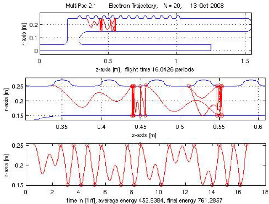
Fig. 12. Discontinuity of the resonance electron's trajectory with gap 2 cm between ripples, even for 20 impacts.
