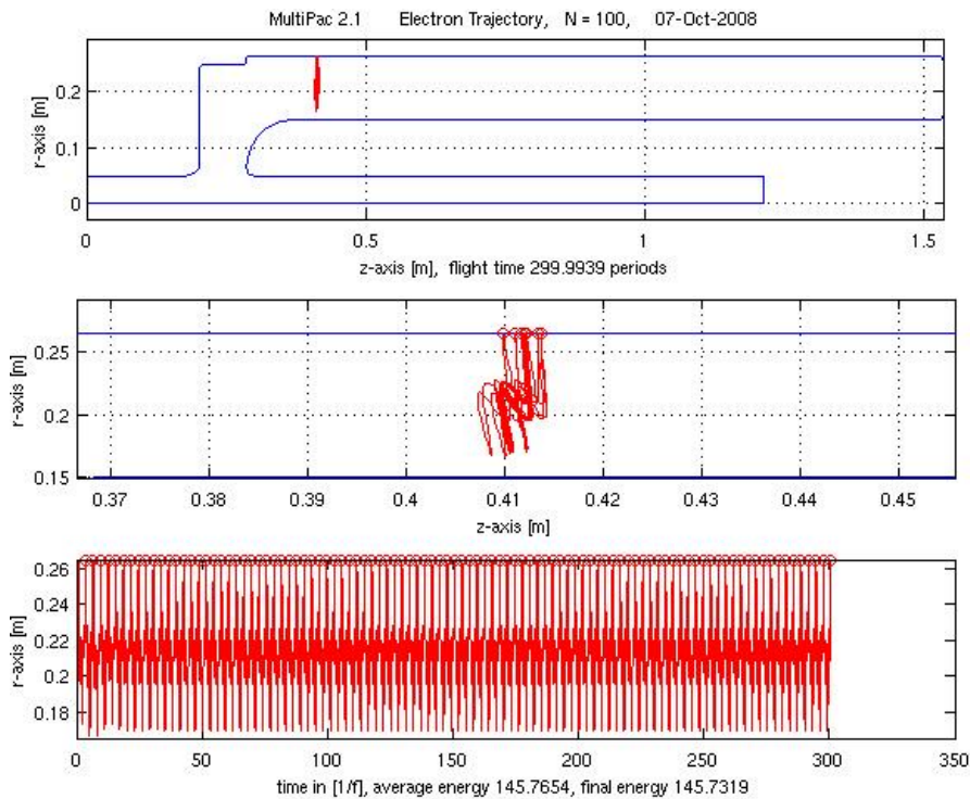
Fig. 7. Multipacting with bigger radius (> 25cm) of outer conductor.
