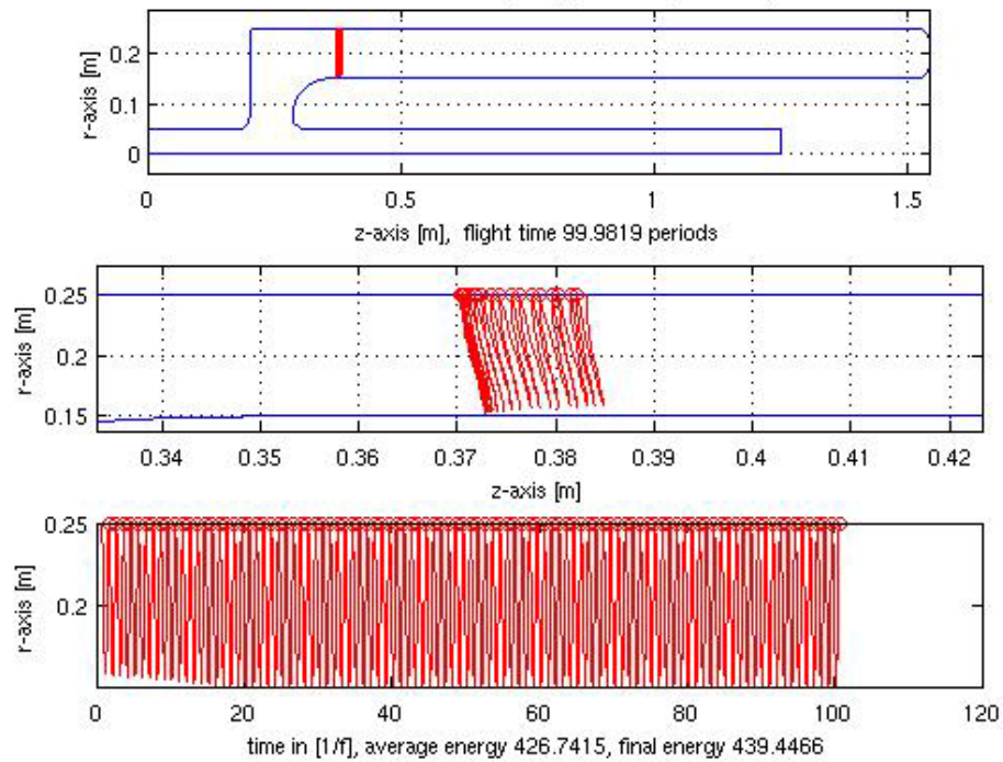
Fig. 4d. Electron trajectory in two-point multipacting at 31 kV/m.
