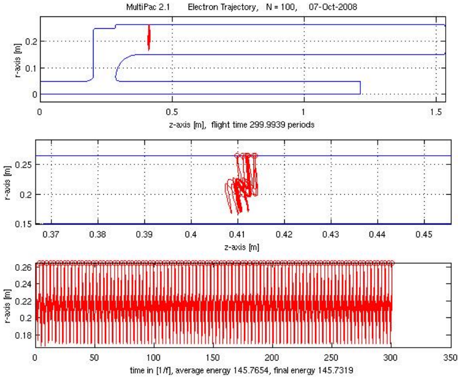
Fig. 7. Multipacting with bigger radius ( > 25\text{cm} ) of outer conductor.
