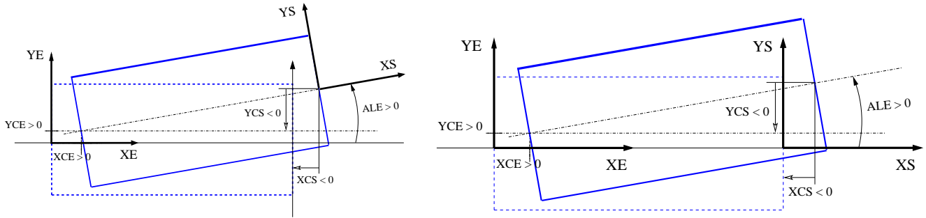
Figure 43: Case of Cartesian frame optical element. Left : moving an optical element using KPOS = 1 . Right : Mis-aligning an optical element using KPOS = 2 . (X_E, Y_E) and (X_S, Y_S) are respectively the incoming and outgoing reference frames.
