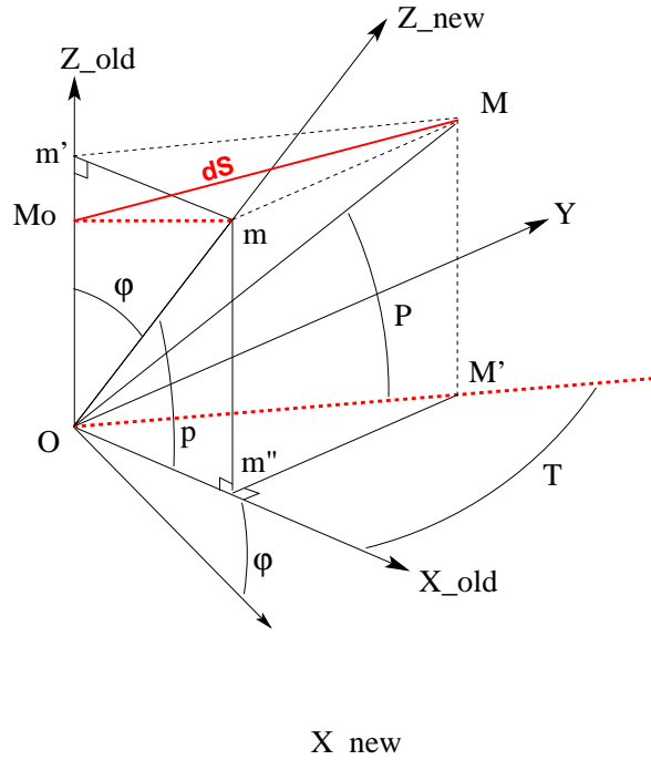
Figure 45: Pitch angle, \varphi , in the “YR” type of rotation, using KPOS=4 . M is the new position, in the rotated plane (Y, Z_{new}) , of a particle with velocity \vec{v}/M_o \vec{M} located at former position M_o in the old, (Y, Z_{old}) , plane. M' , m , m' are projections of M , m'' is projection of M' . T and P are the horizontal and vertical angles as defined in Fig. 1. p is the projection of P .
