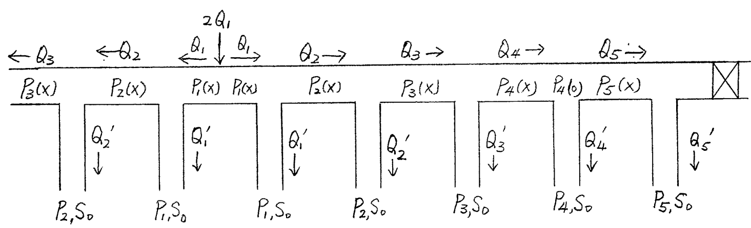
Fig. 1 (a). Schematics of AGS Ring Vacuum Chamber. w/ uniform outgassing
