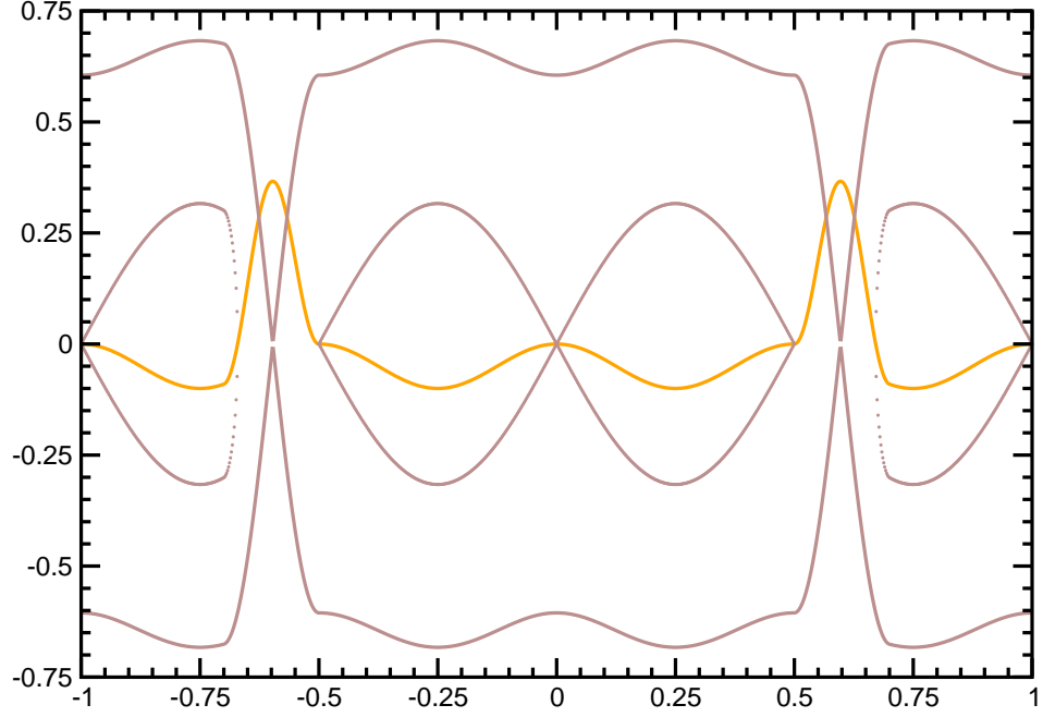
Figure 4: Here the orange curve is -U(\phi) from Figure 3 . The outer brown curves are the separatrices that pass through unstable fixed points \phi_u = \pm 0.5970\pi . These curves form the barrier bucket. The inner brown curves are the separatrices that pass through the unstable fixed points \phi_u = 0, \pm\pi/2, \pm\pi . These curves form the harmonic 4 buckets. Note that the barrier bucket is distorted by the harmonic 4 voltage, as are two (the left-most and right-most) of the harmonic 4 buckets by the barrier bucket voltage. The horizontal axis is \phi/\pi .
