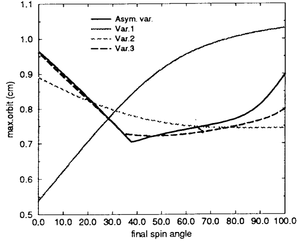
Figure 5: The maximum orbit deviation values on the spin direction angle after the rotator for all considered designs at fixed energy \gamma = 100 .
