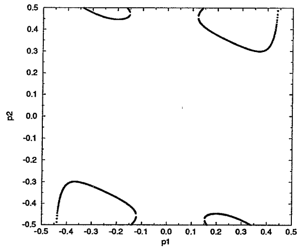
Figure 4: The relationship between the fields, p_1 and p_2 , of first and second helical magnets.
