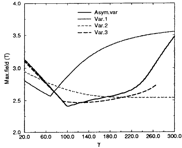
Figure 6: The maximum value of magnetic field required at given energy to provide the longitudinal polarization in IP.
