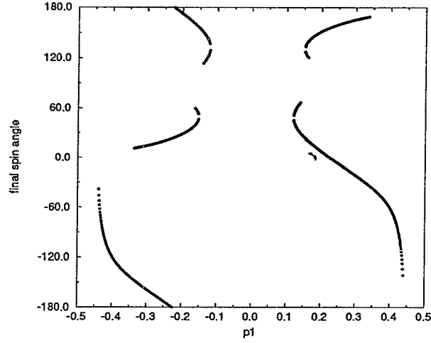
Figure 3: The relationship between the spin direction angle after the rotator and the field p_1 of first magnet.
