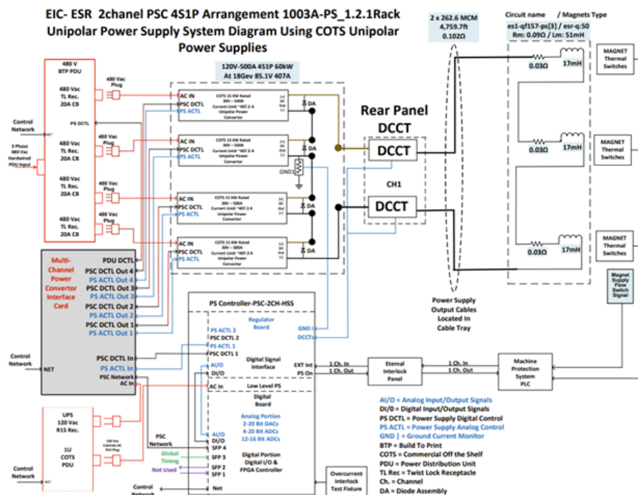
Figure 25. 4S1P Unipolar Power Supply Rack Configuration
