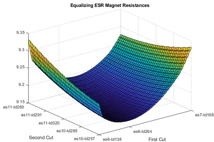
Figure 16. Surface plot of segment resistances
