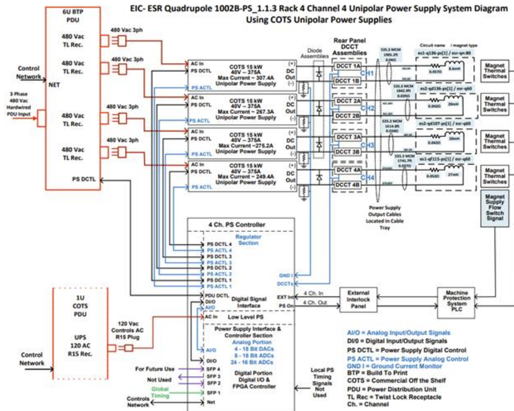
Figure 24. Single Unipolar Power Supply Rack Configuration
