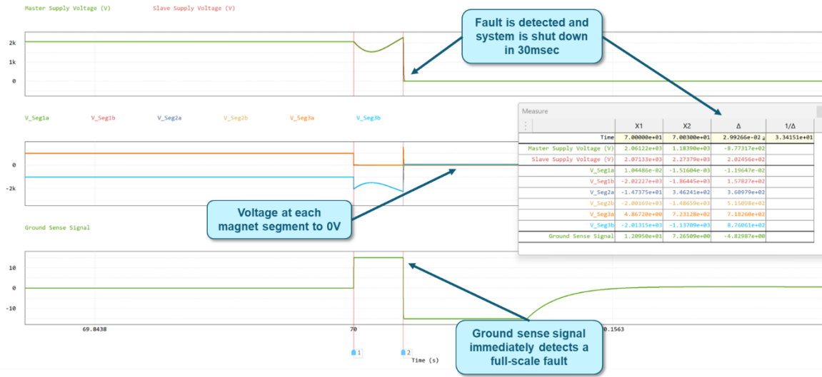
Figure 23. ESR main dipole simulation results from a direct short
