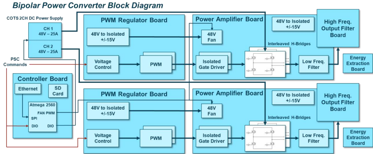
Figure 33. ESR Corrector BTP BPC Block Diagram
