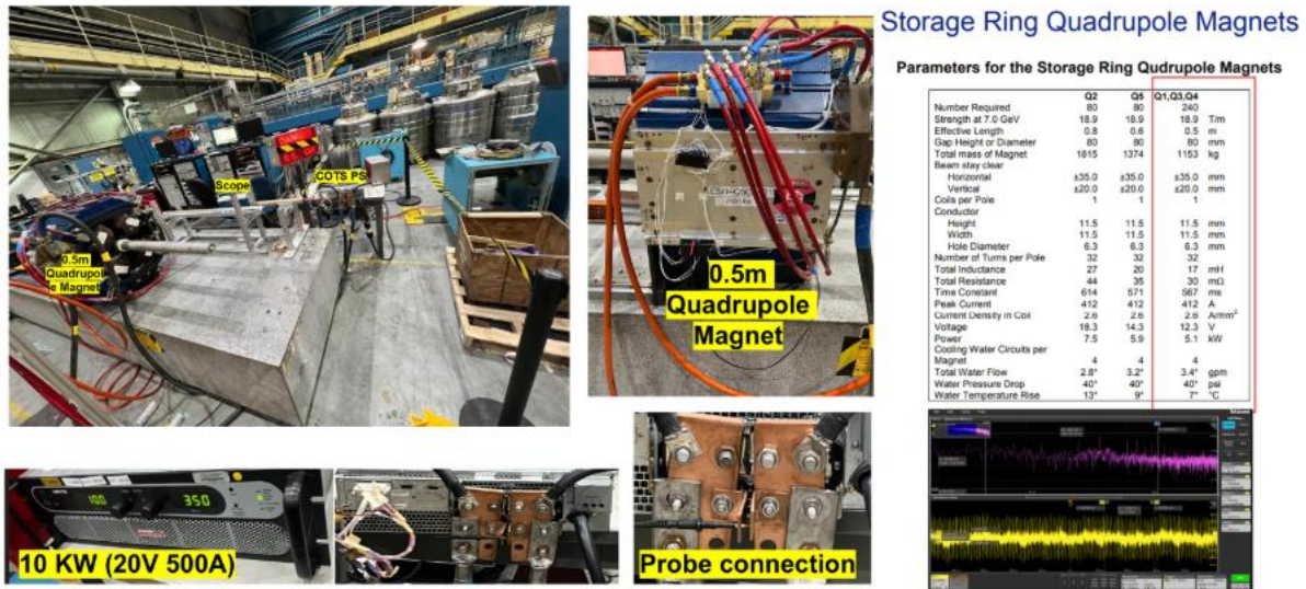
Figure 30. In-house Ripple Testing with Q50 Equivalent Magnet
