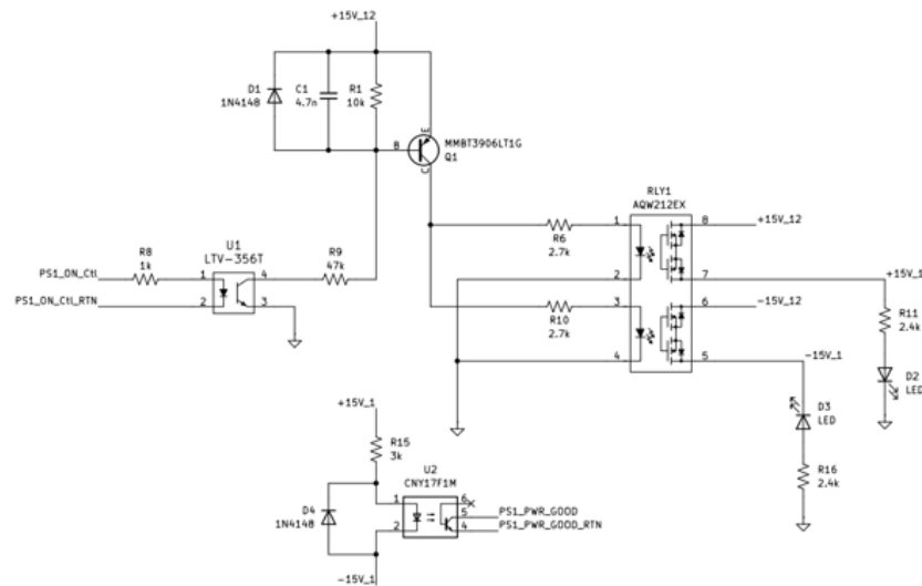
Figure 40. ESR Dipole Trim BTP BPC On-Command and Readback Circuit
