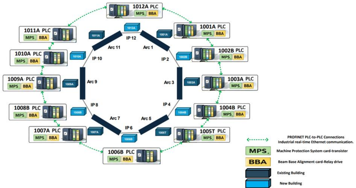
Figure 49. Distributed PLC Architecture across ESR buildings showing PROFINET Communication and Integration of MPS and BBA Modules
