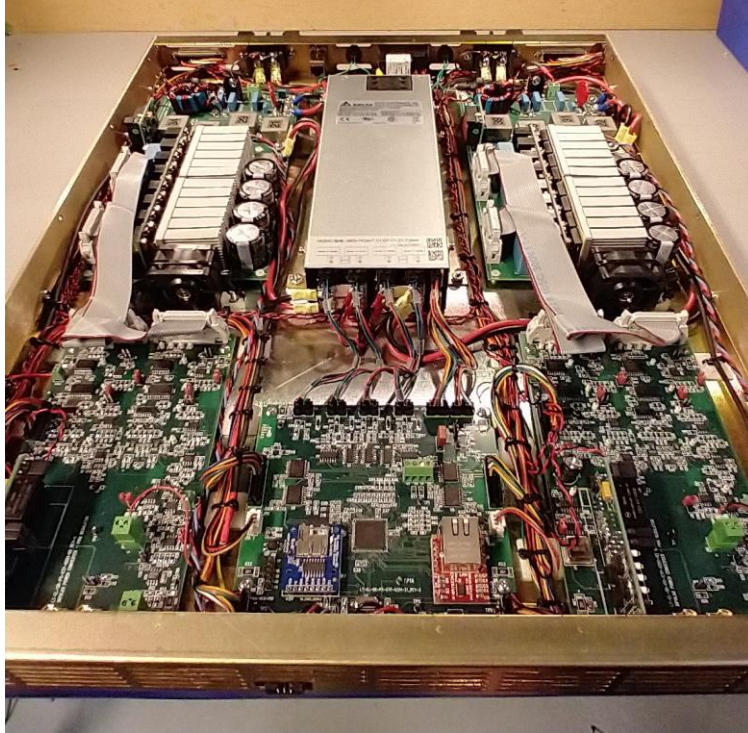
Figure 32. NSLS-II BPC-2CH-5-16V-35A
