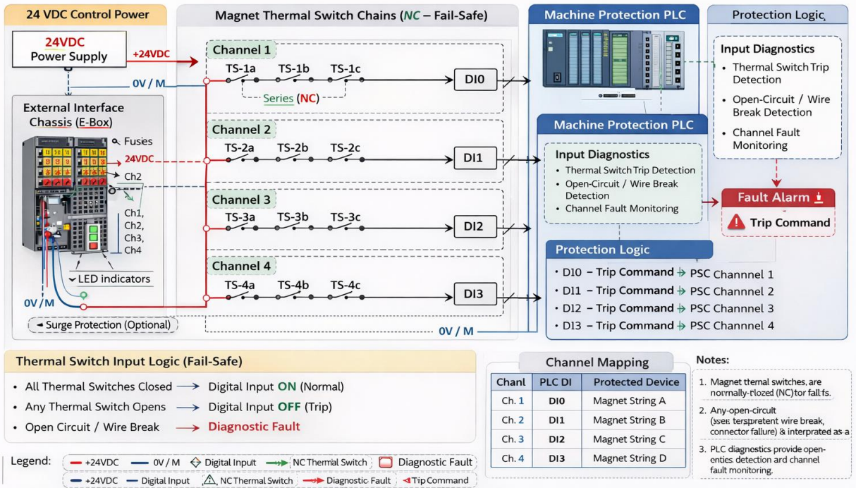
Figure 52. PLC-based interlock architecture showing thermal switch chains, diagnostics, and trip logic
