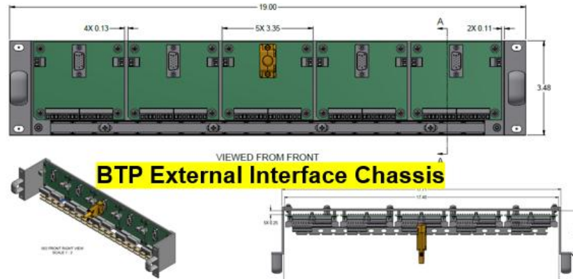
Figure 51. External Interface Chassis
