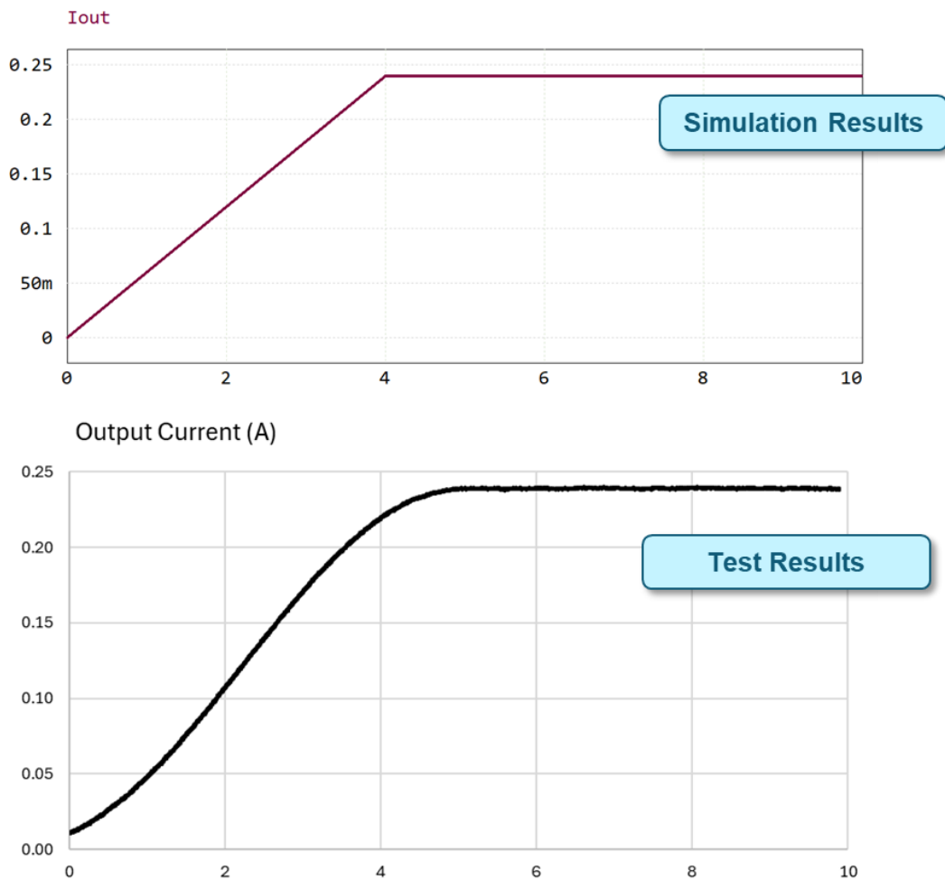
Figure 44. ESR Dipole Trim BTP BPC Simulation VS. Prototype Test Results
