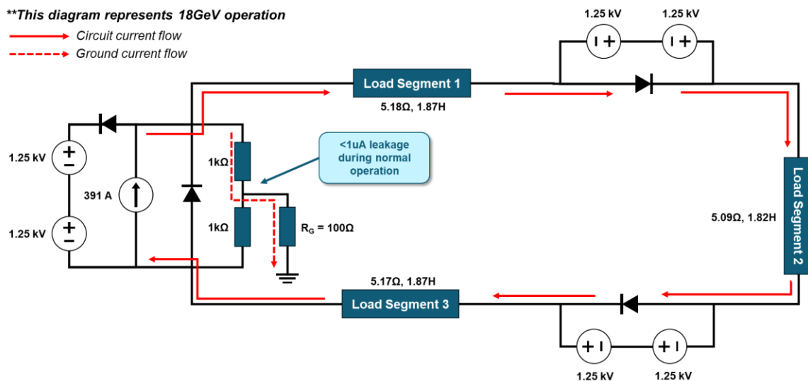
Figure 20. Block Diagram of ESR Main Dipole During Normal Operation
