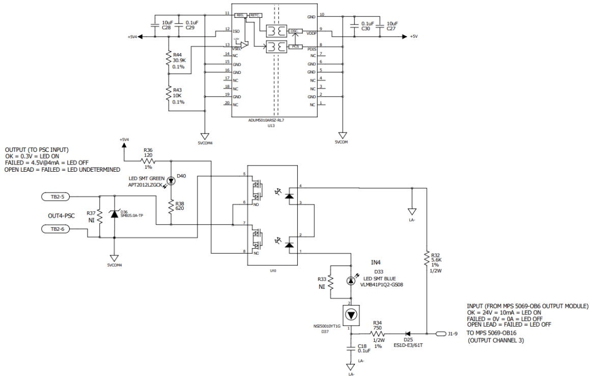
Figure 53. Solid-State Relay (SSR) Based Isolated Interface Between PLC and PSC
