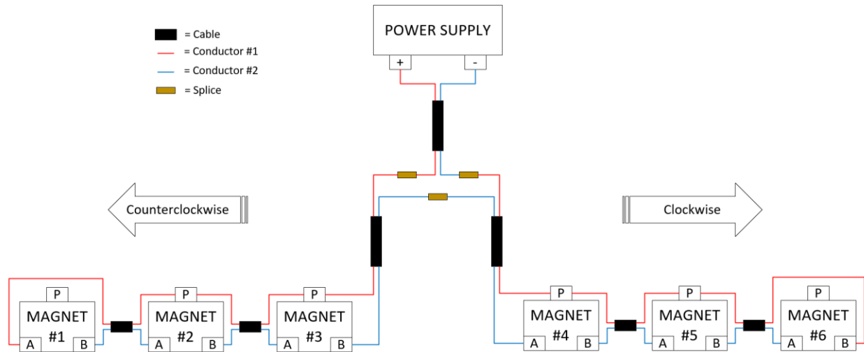
Figure 57. Cable Routing with Power Supply Inside of Magnet String Span
