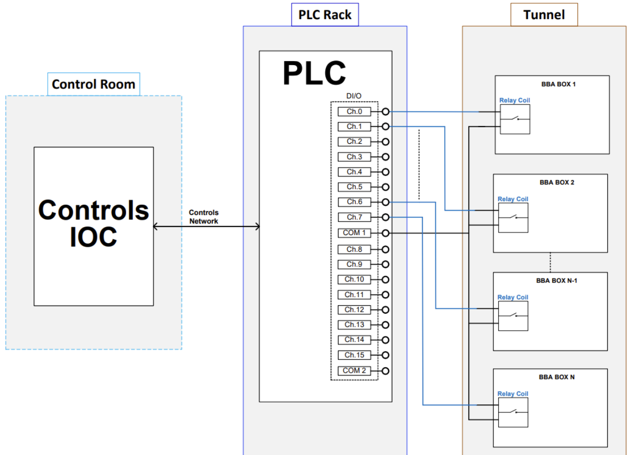
Figure 55. PLC integration for BBA showing relay control, IOC interface, and connection to multiple BBA units
