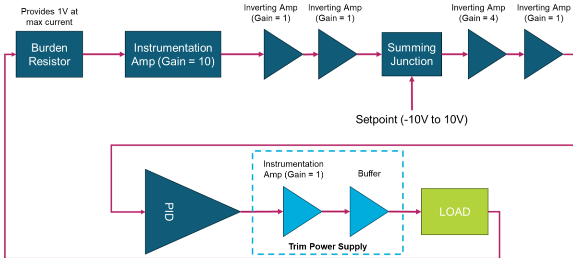
Figure 39. ESR Dipole Trim BTP BPC Block Diagram
