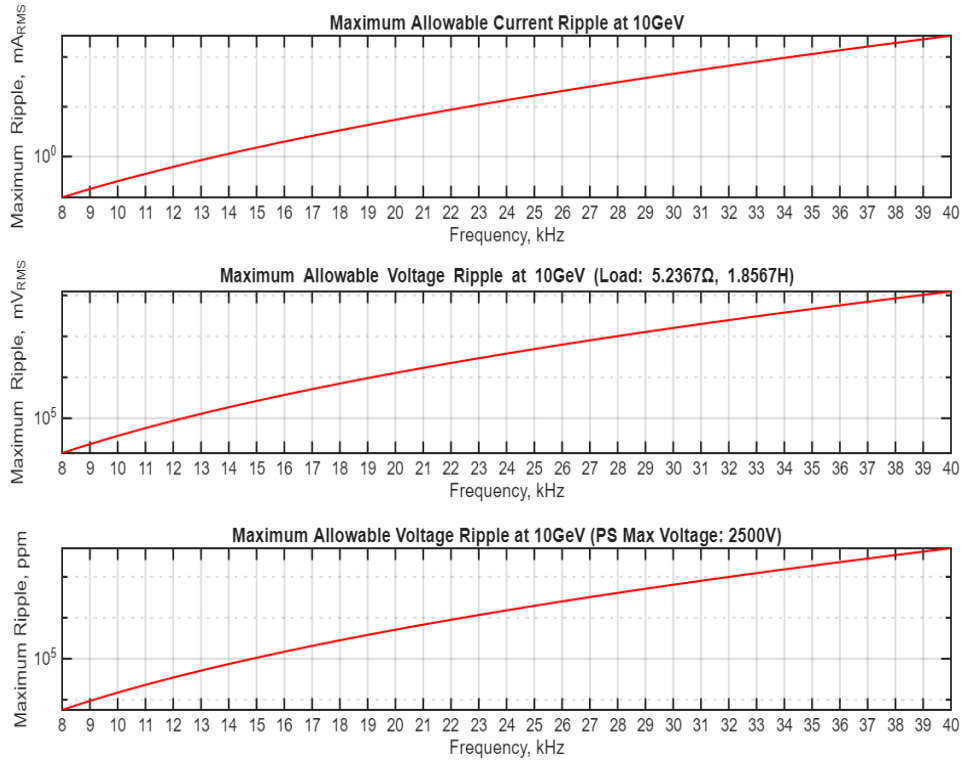
Figure 2. Maximum Allowable Ripple for ESR Main Dipole Power Supplies from 8kHz-40kHz. 10GeV operating conditions produce the tightest specification and are therefore used to generate the plots.
