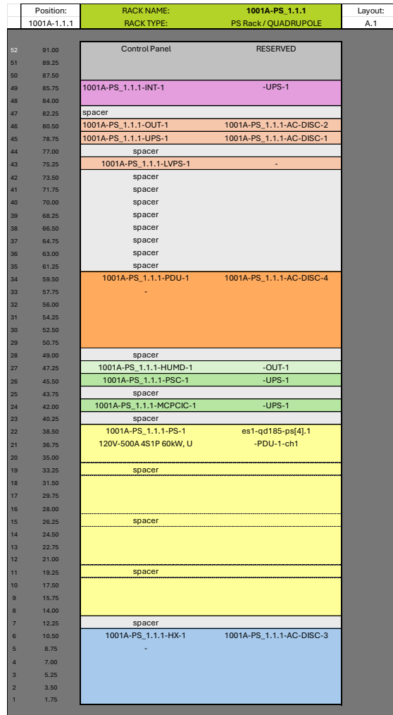
Figure 11. Individual Rack Layout
