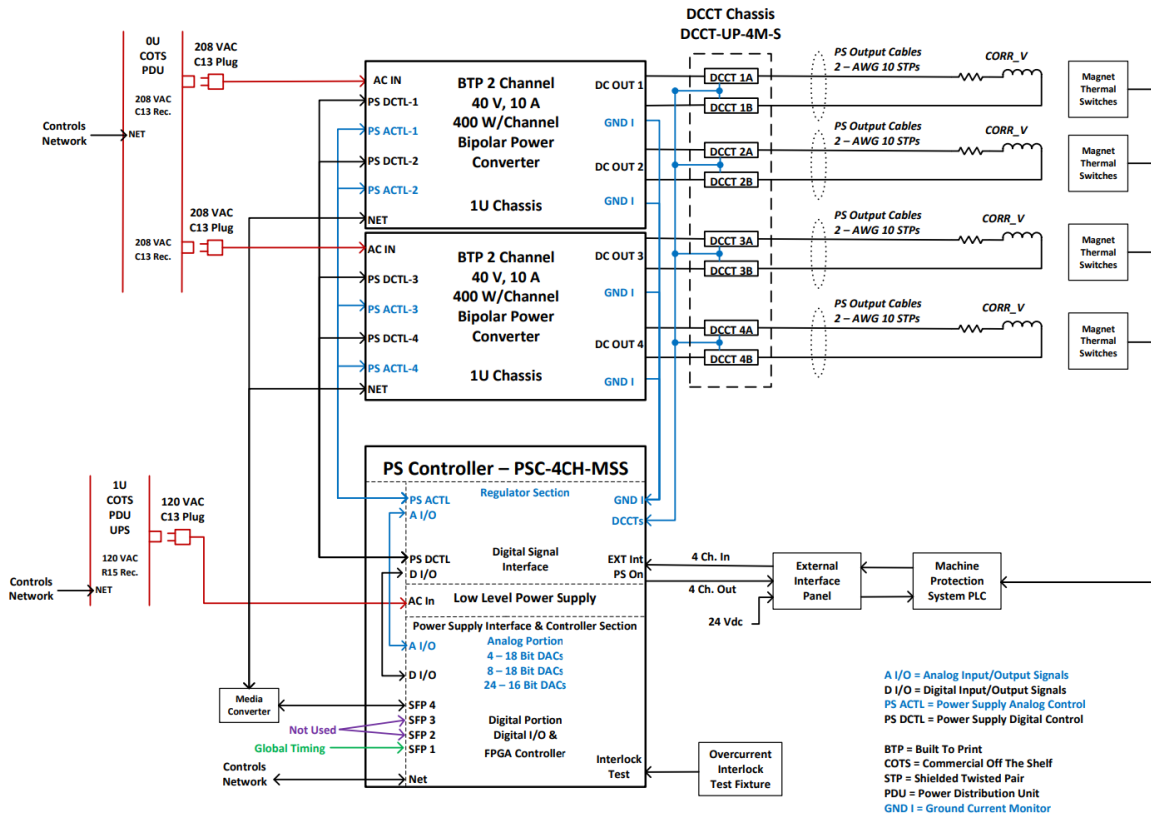
Figure 38. ESR Corrector BPCs Interfacing with Auxiliary Equipment in a Rack
