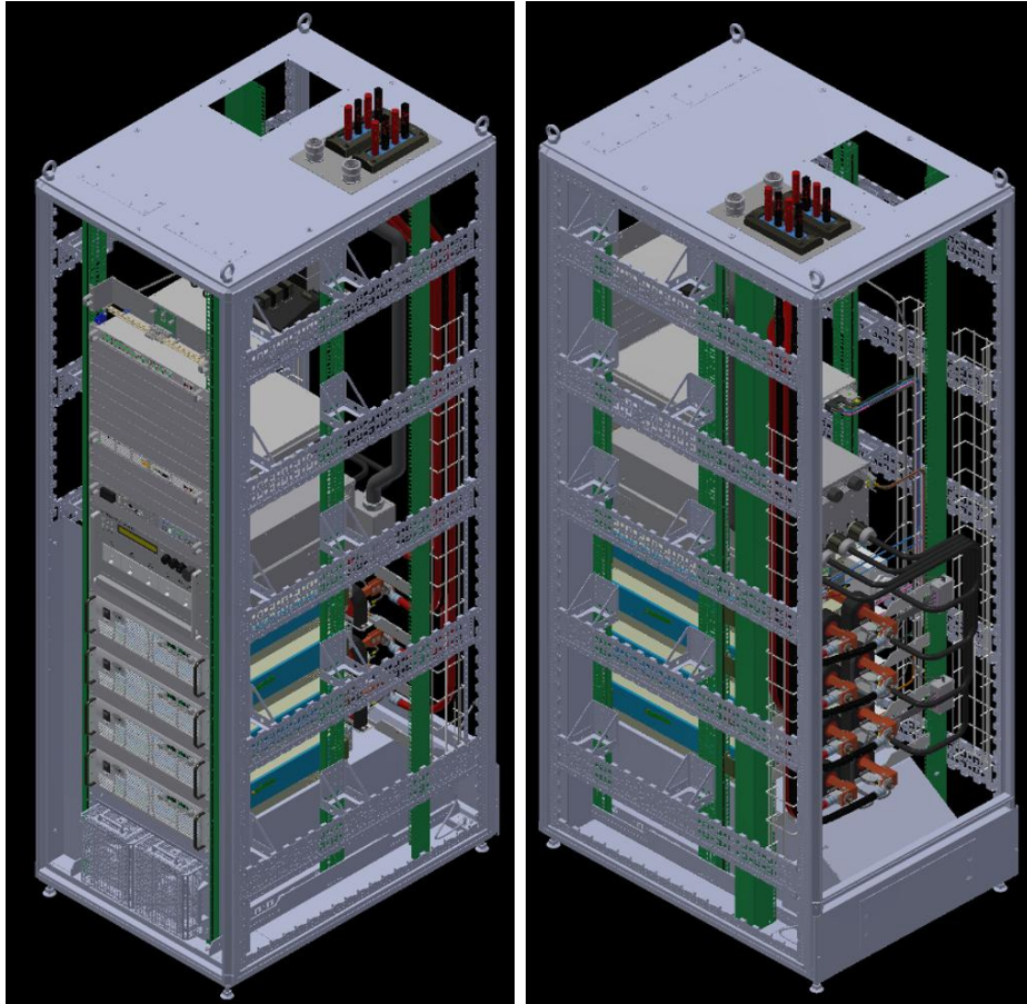
Figure 27. 3D Rack Model
