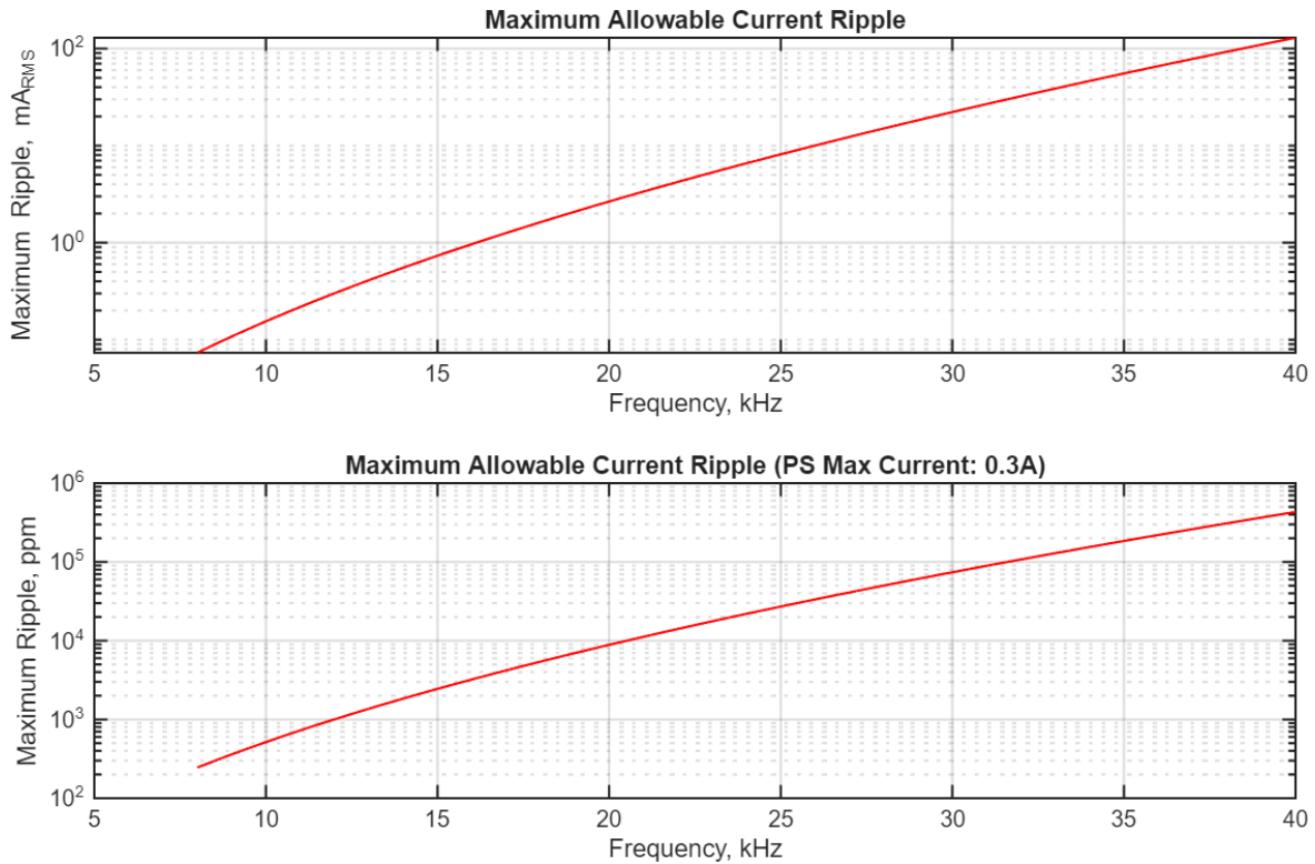
Figure 3. Maximum allowable ripple for ESR Dipole Trim coils
