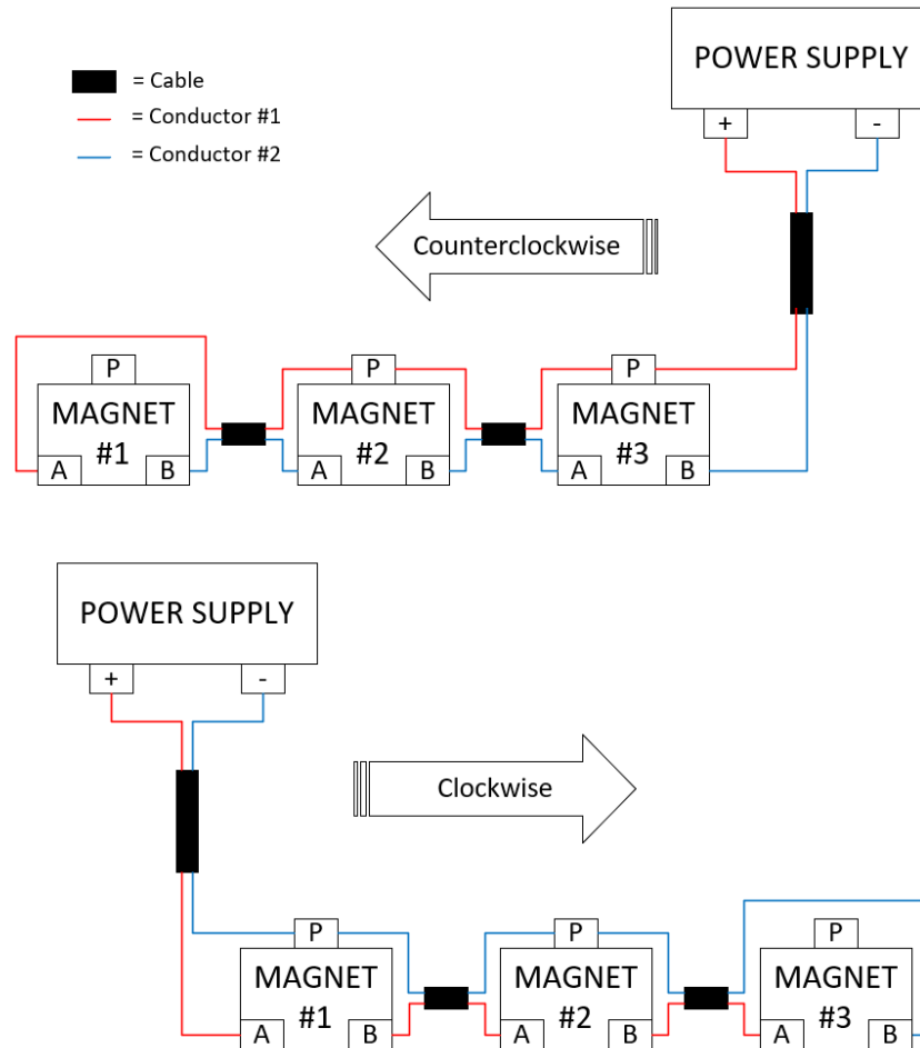
Figure 56. Cable Routing with Power Supply Outside of Magnet String Span
