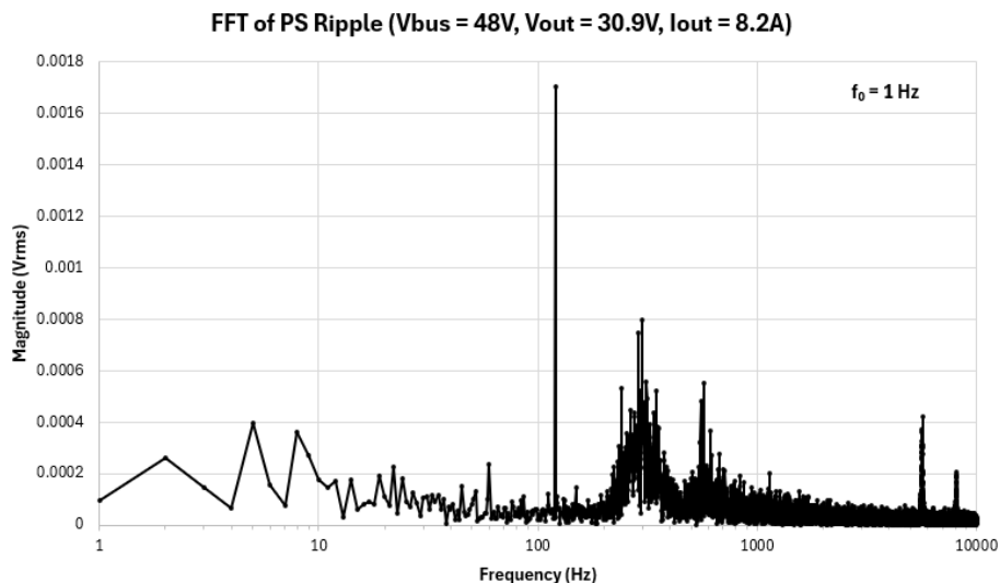
Figure 43. FFT of BPC Voltage Ripple under ESR Corrector Power Supply Operating Conditions
