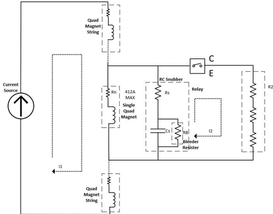
Figure 47. BBA System Block Diagram showing magnet and shunt resistor
