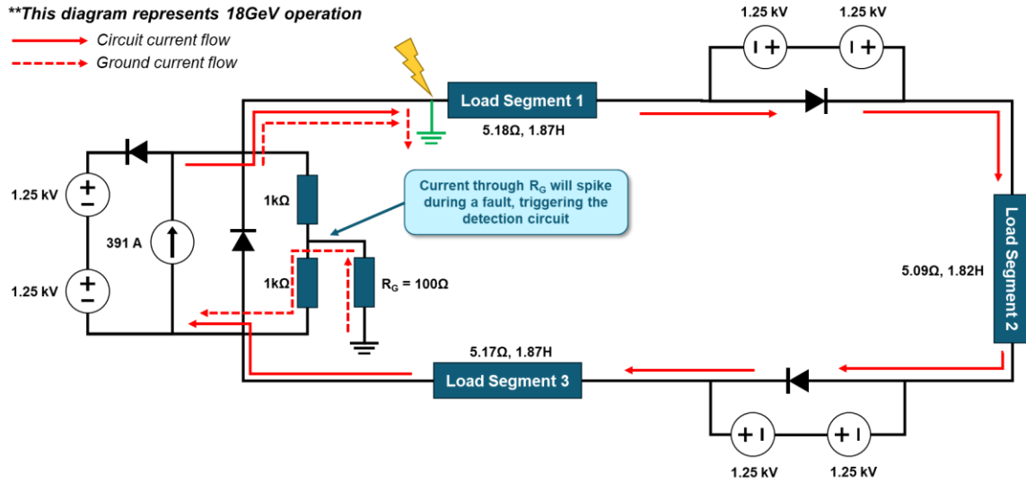
Figure 21. Block Diagram of ESR Main Dipole during Ground Fault Condition
