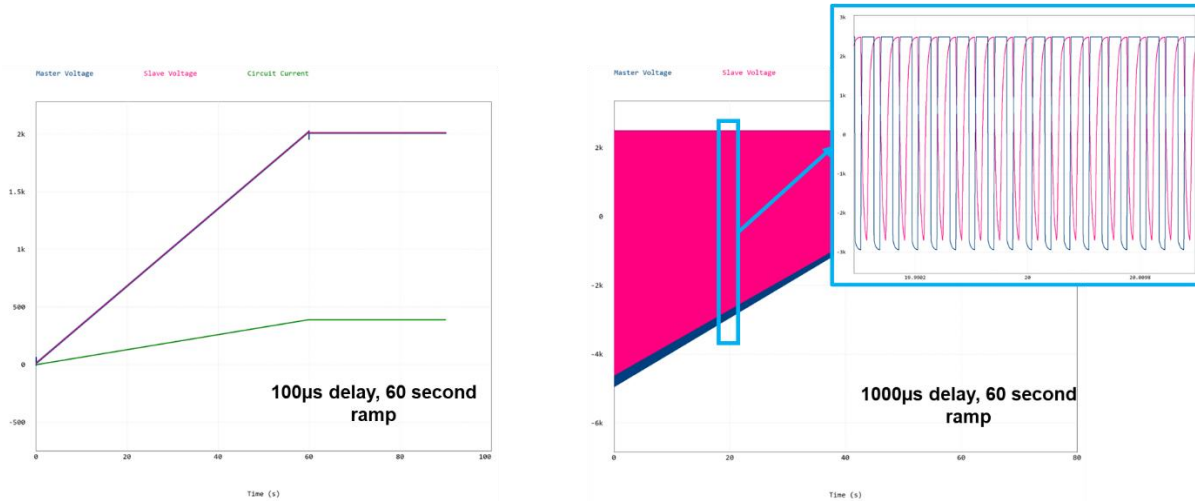
Figure 19. Effect of Transmission Latency on ESR Main Dipole Circuit
