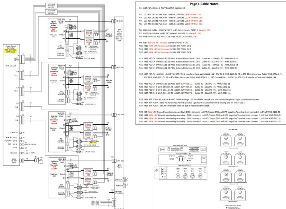
Figure 26. Interconnecting Wiring Block Diagram
