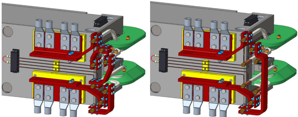
Figure 15. Example of a D13 magnet with 12-turn tap configuration (left) and 5-turn tap configuration (right)
