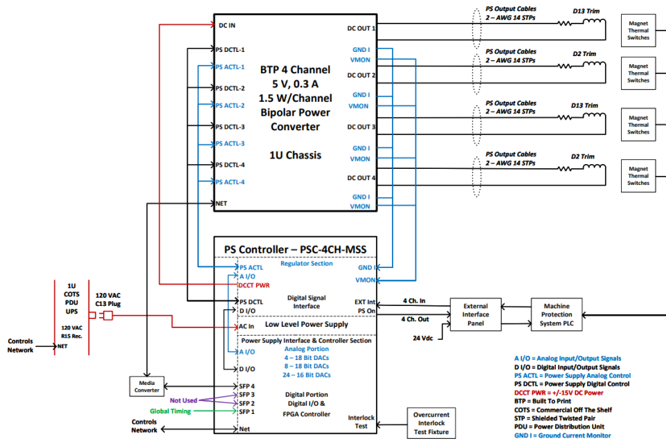
Figure 42. ESR Dipole Trim BPCs Interfacing with Auxiliary Equipment in a Rack
