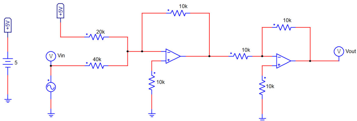
Figure 36. Output Voltage Feedback to Controller Board Circuit
