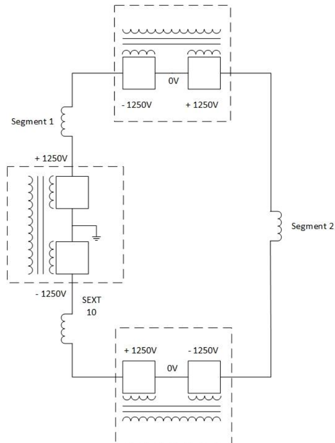
ESR Main Dipole Topology 7500V 700A
