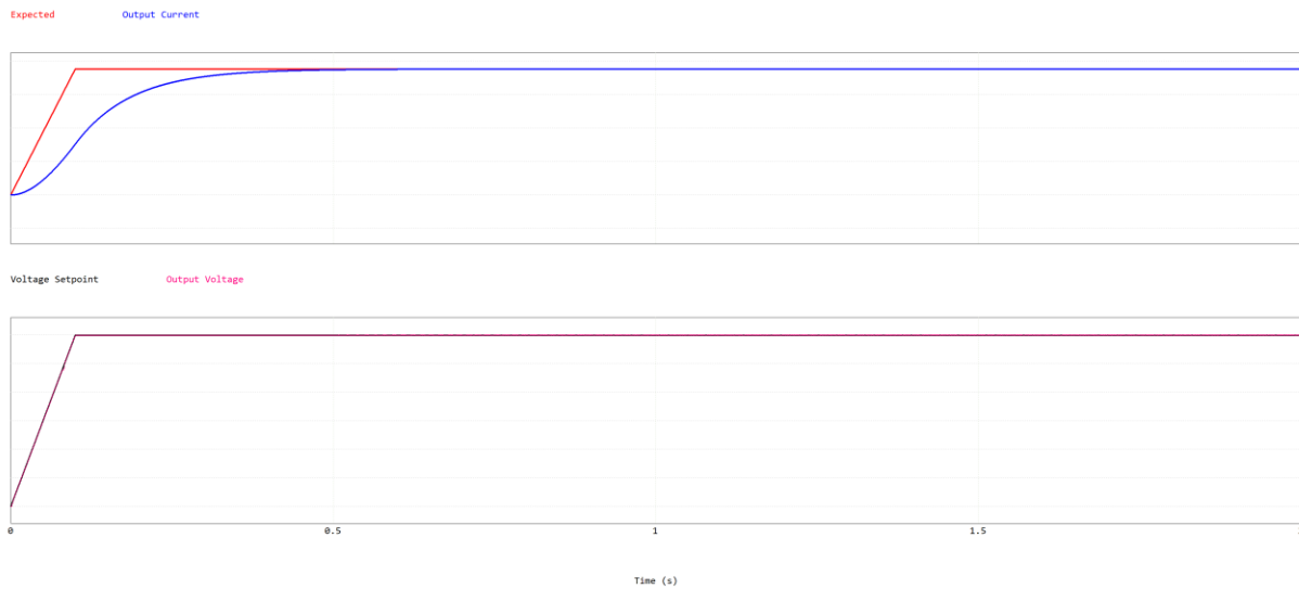
Figure 35. Output Voltage and Current of BPC Simulation (Vertical Corrector Load)
