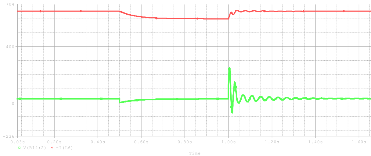
Figure 48. Simulation Showing Spikes in magnet during BBA excitation. RED is Magnet current and green is Magnet Voltage, spike is +250V/-50V, decaying sinewave, about 40HZ
