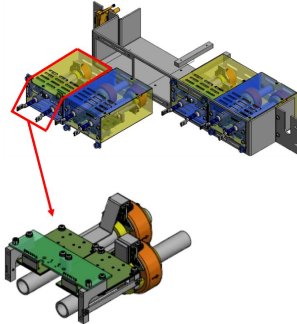
Figure 46. BTP DCCT Chassis
