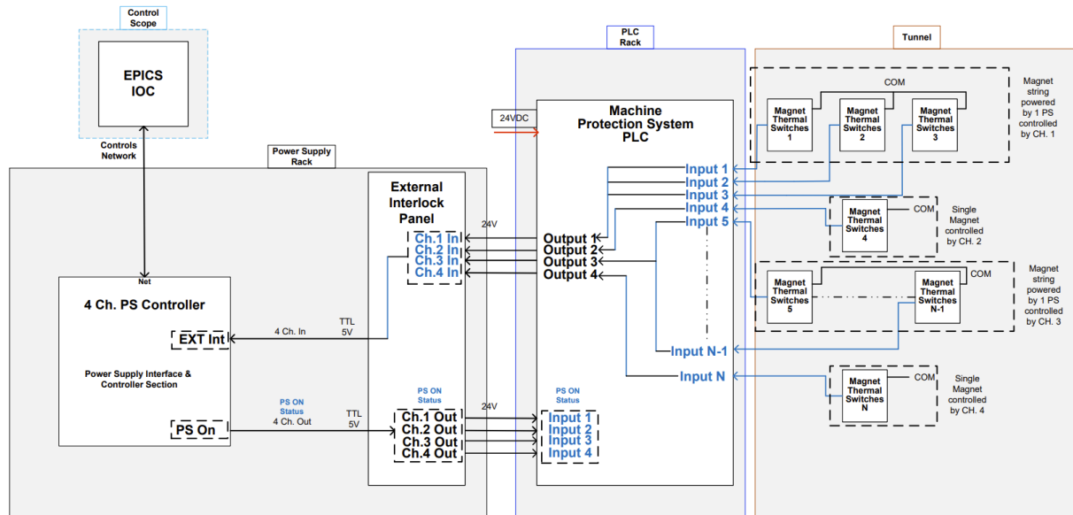
Figure 54. End-to-end interlock system showing signal flow from magnet thermal switches to PLC and PSC shutdown
