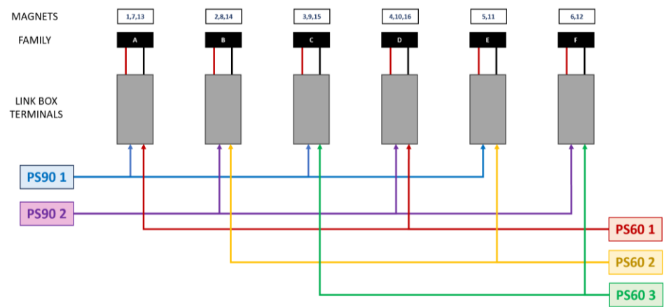
Figure 7. General layout for sextupole families (symmetrical across all arcs)
