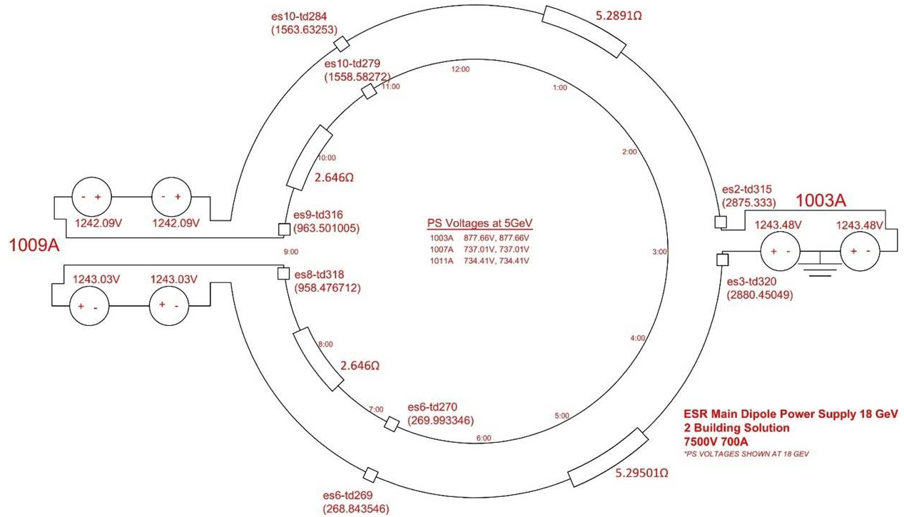
Figure 17. Voltage Balanced ESR Main Dipole Circuit (18 GeV)
