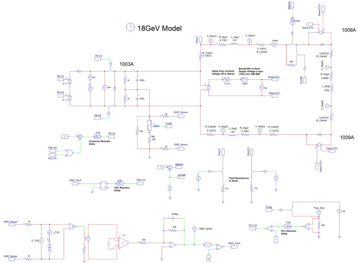
Figure 22. PSIM Model of ESR Main Dipole Circuit
