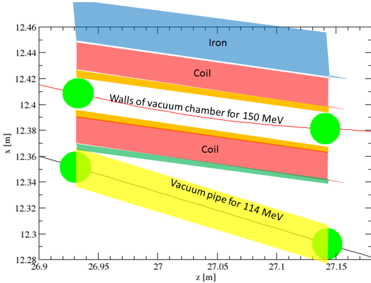
Figure A1. The schematic diagram of the cross section at the median plane of the S4.BEN01 electromagnet. The thin traces on the figure are the trajectories of the reference particles for the 114 and 150 MeV electron bunches. The center of the green circles on the figure represent the reference particles of the 114, and 150 MeV bunches at the entrance and exit of the magnet. The red areas represent the coil of the magnet. The walls of the vacuum chamber are the thin orange stripes, and the green stripe is the coil-retaining nonmagnetic sheet. The yellow quadrilateral region is the vacuum pipe of the 114 MeV beam.
